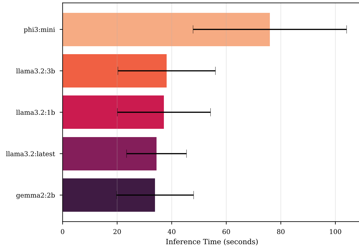
Average Inference Time by Model
