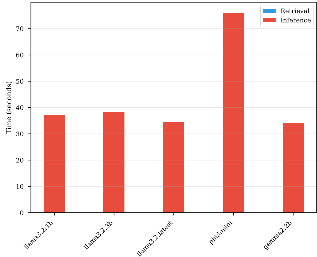
Response Time Breakdown
