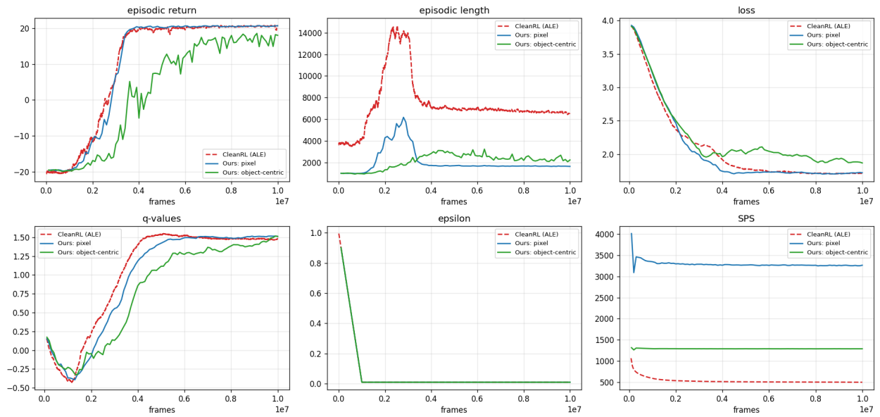
C51 on pong: ours (pixel + object-centric) vs CleanRL c51_atari_jax
