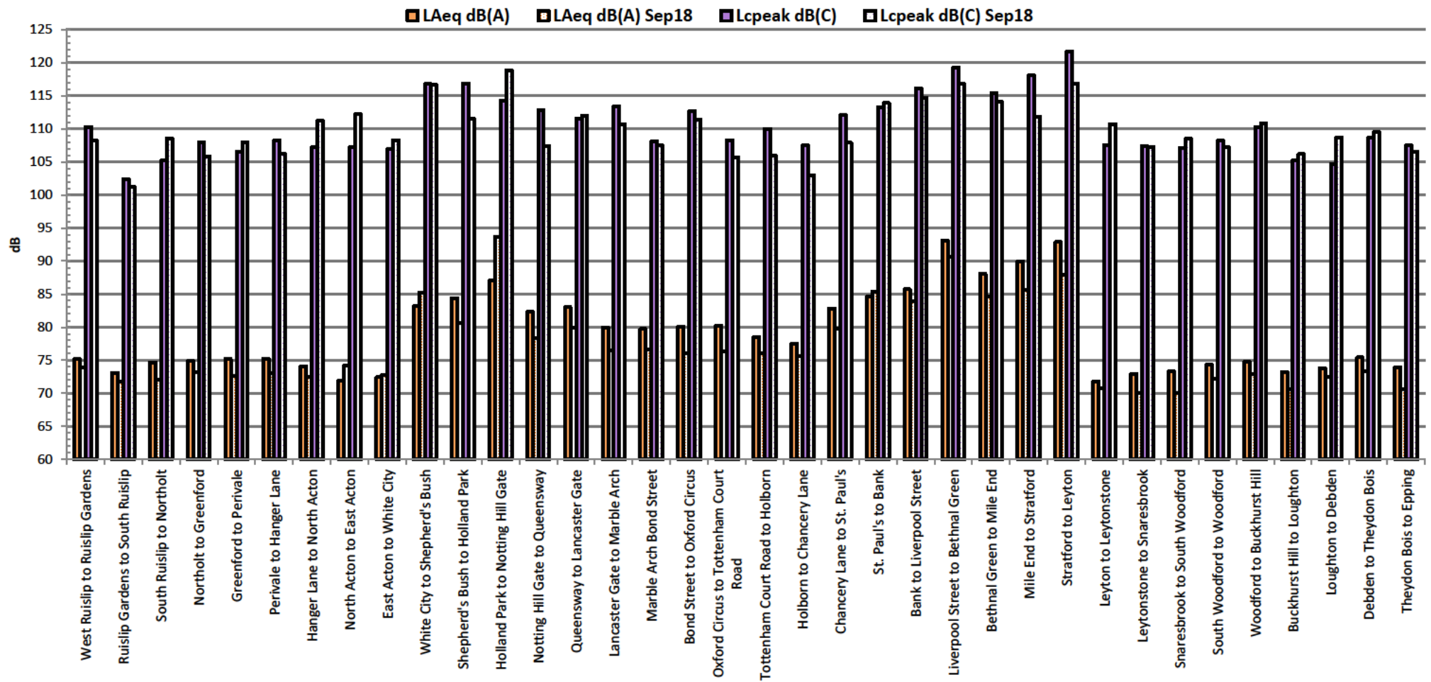
Chart 2 – Average weighted noise levels, on the Central eastbound, between West Ruislip and Epping
