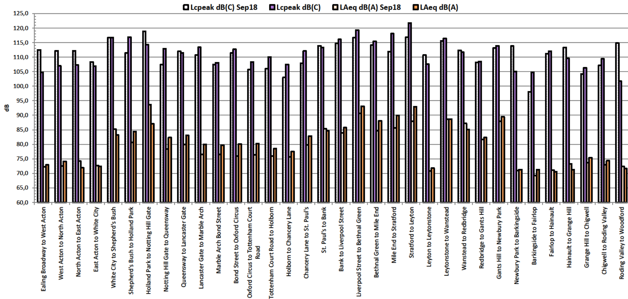
Chart 1 - Average weighted noise levels on the Central eastbound road, between Ealing Broadway and Woodford, via Newbury Park
