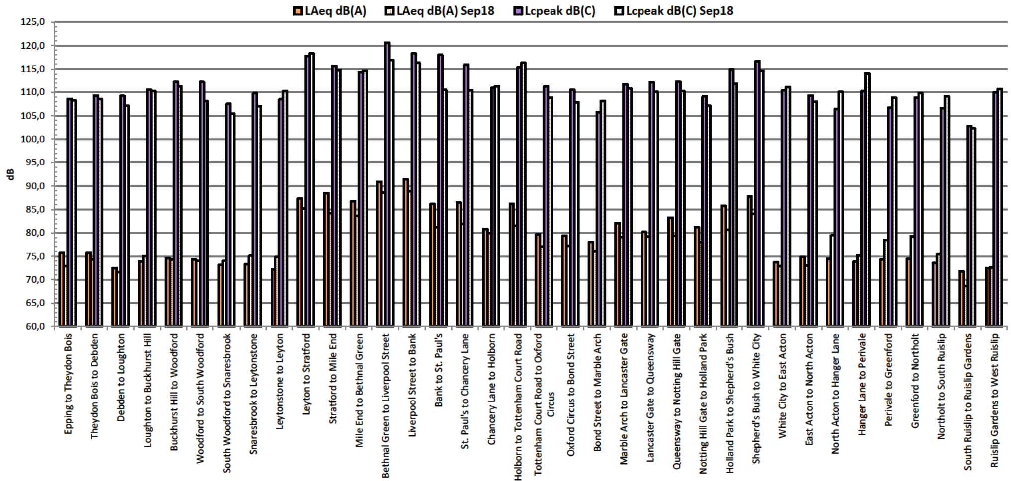
Chart 4 – Average weighted noise levels, on the Central westbound road between Epping and West Ruislip
