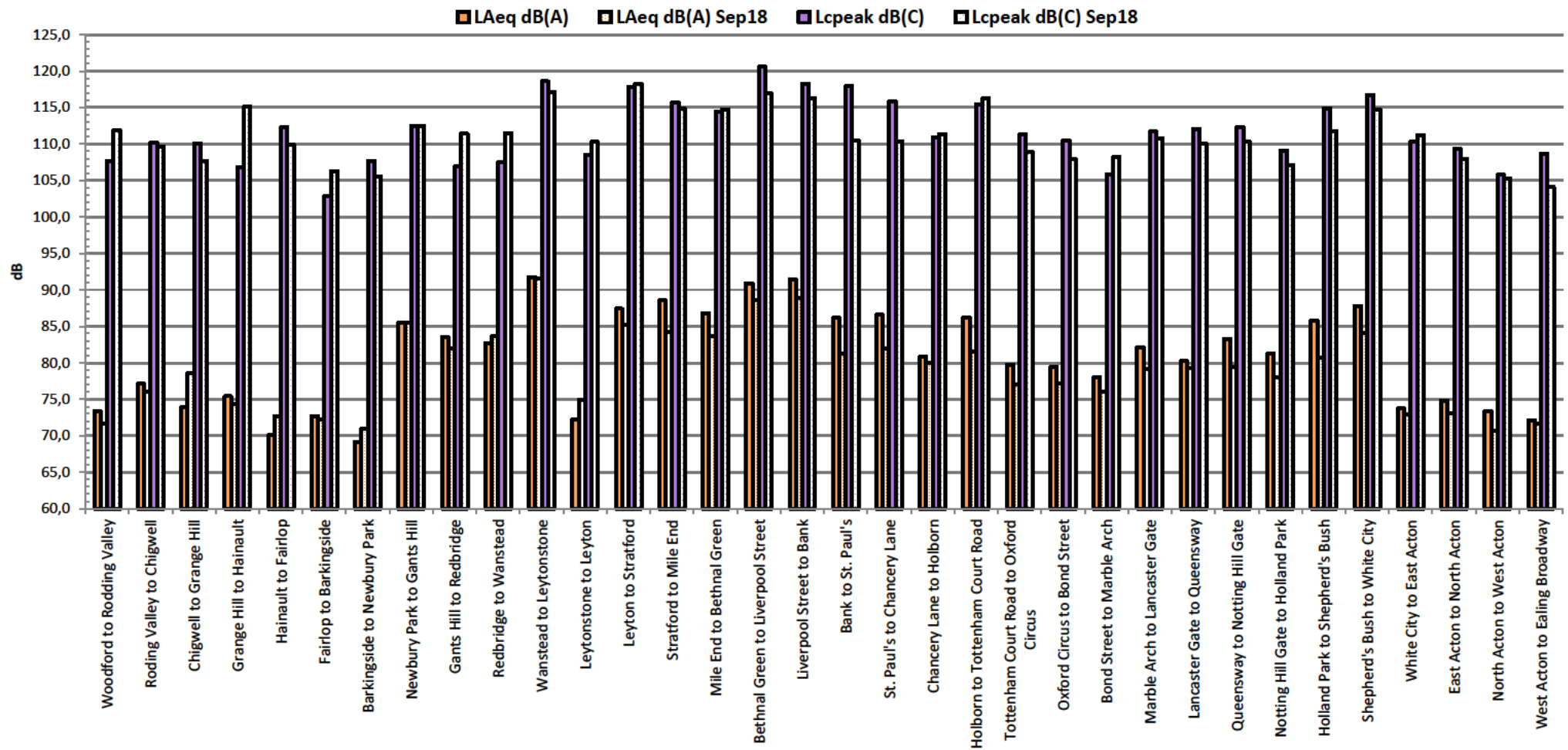
Chart 3 – Average weighted noise levels, on the Central westbound road between Woodford and Ealing Broadway, via Newbury Park
