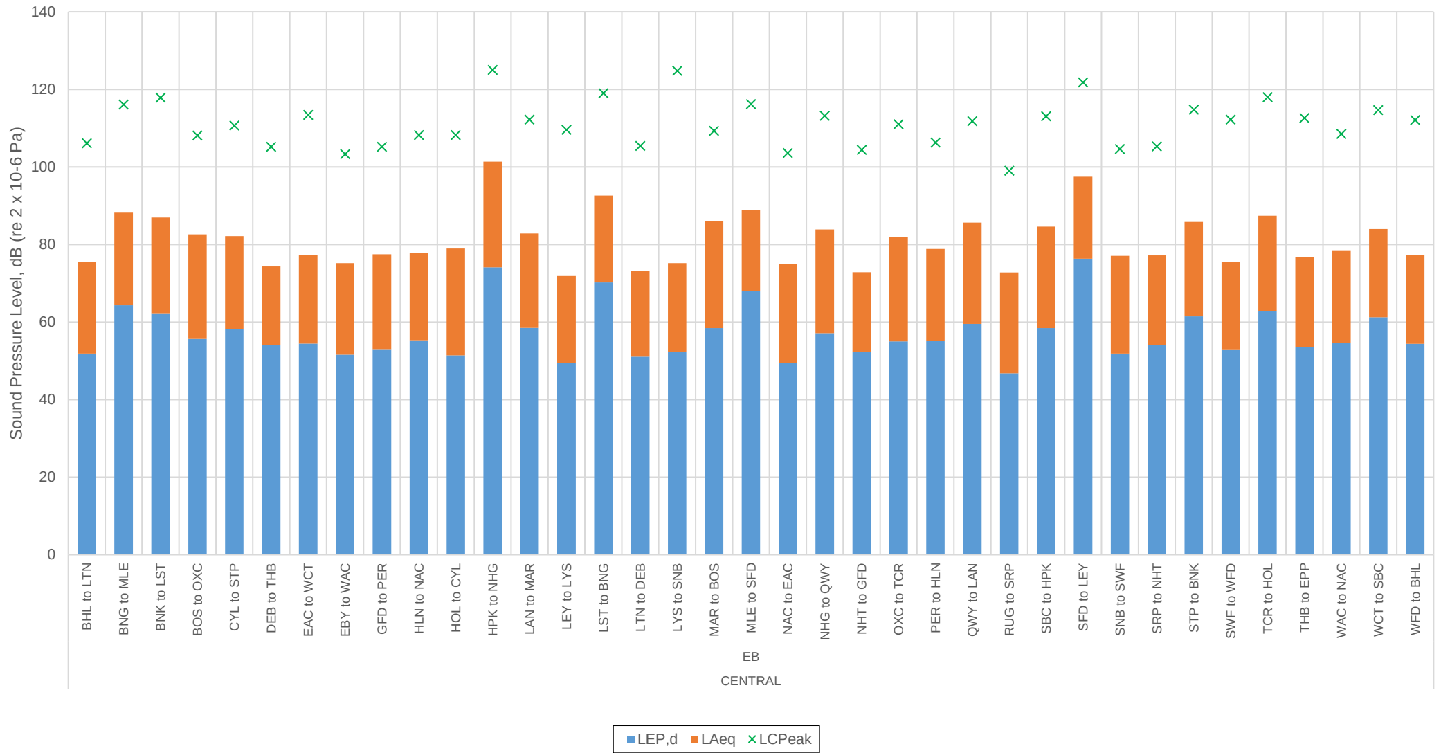
Figure 2 - Interstation noise levels on the Central eastbound
