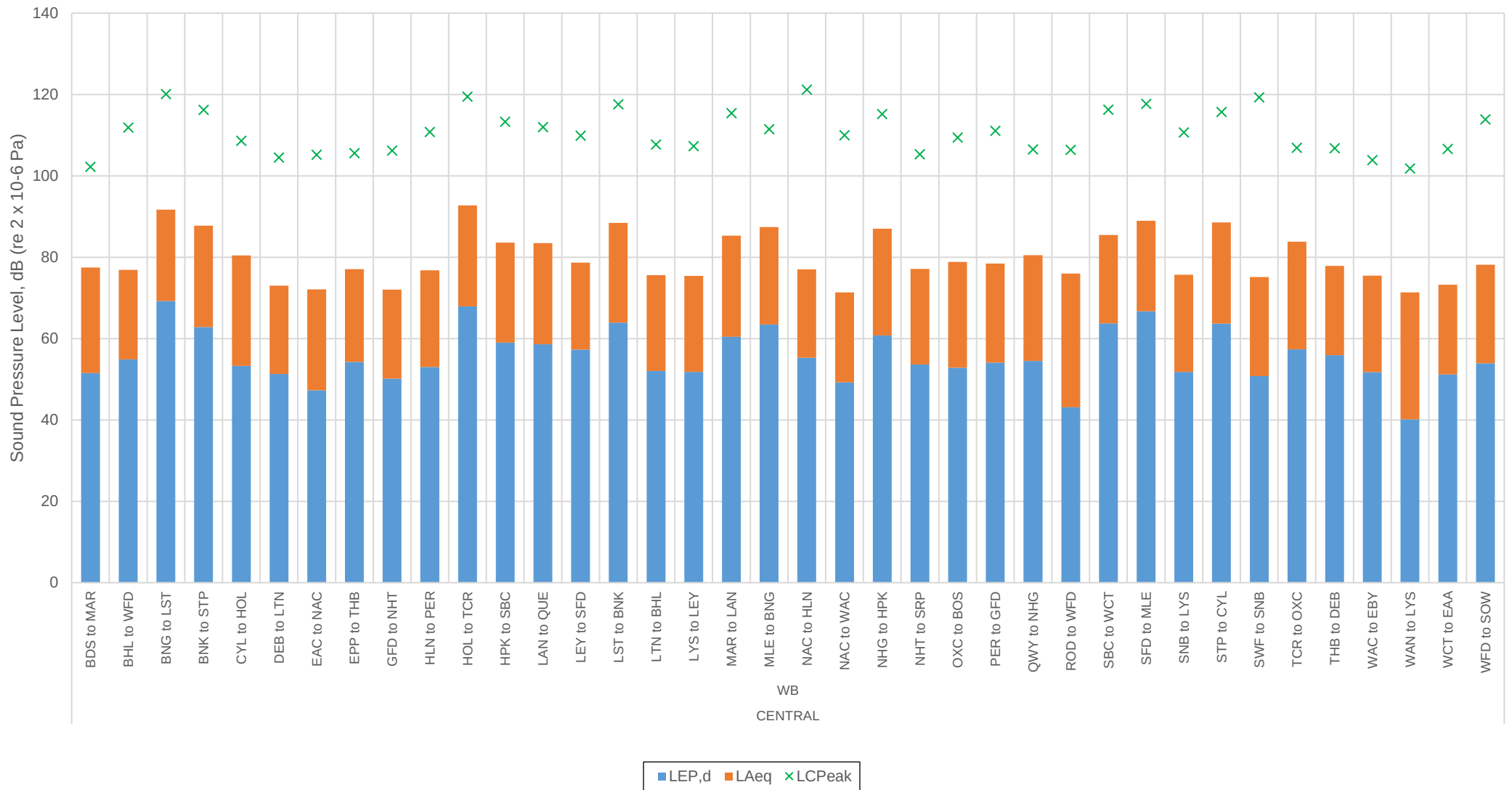
Figure 3 - Interstation noise levels on the Central westbound
