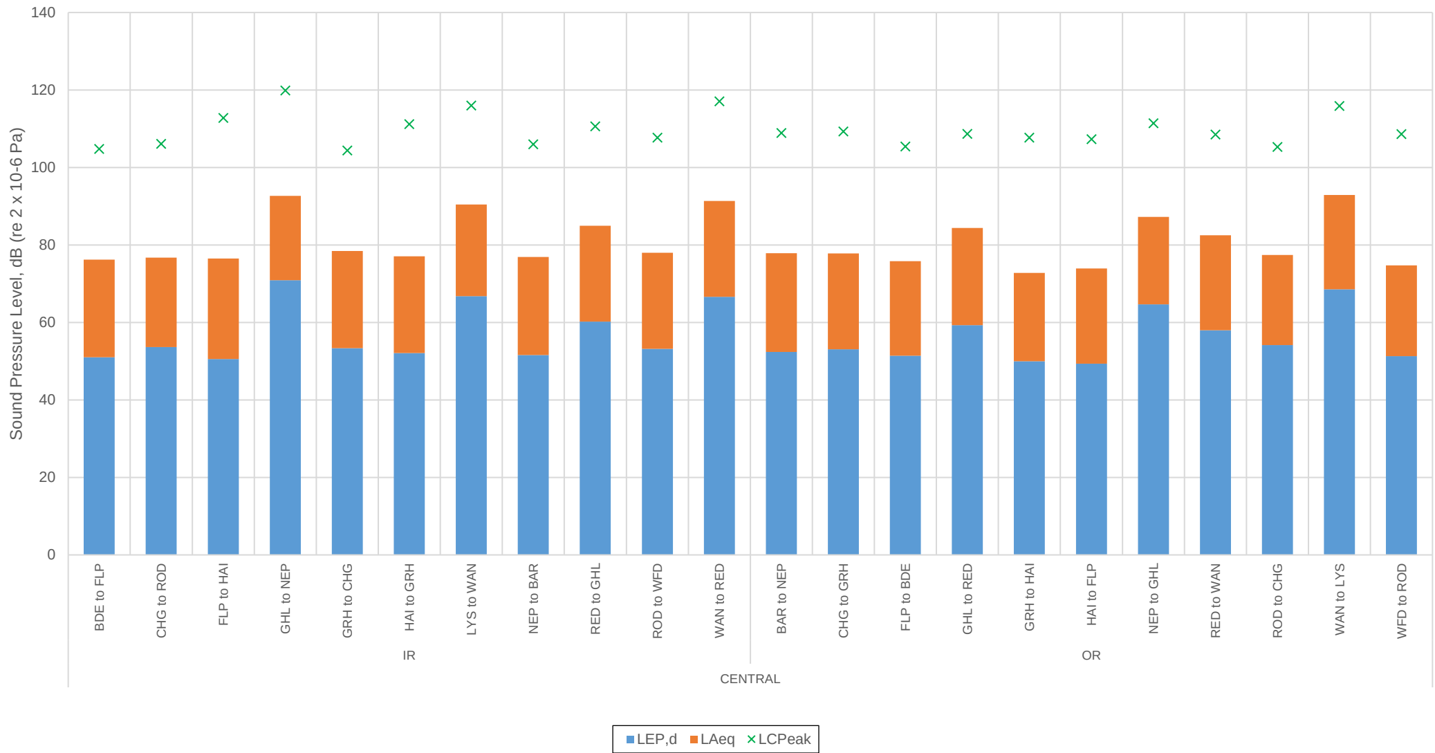
Figure 3 - Interstation noise levels on the Central inner and outer road
