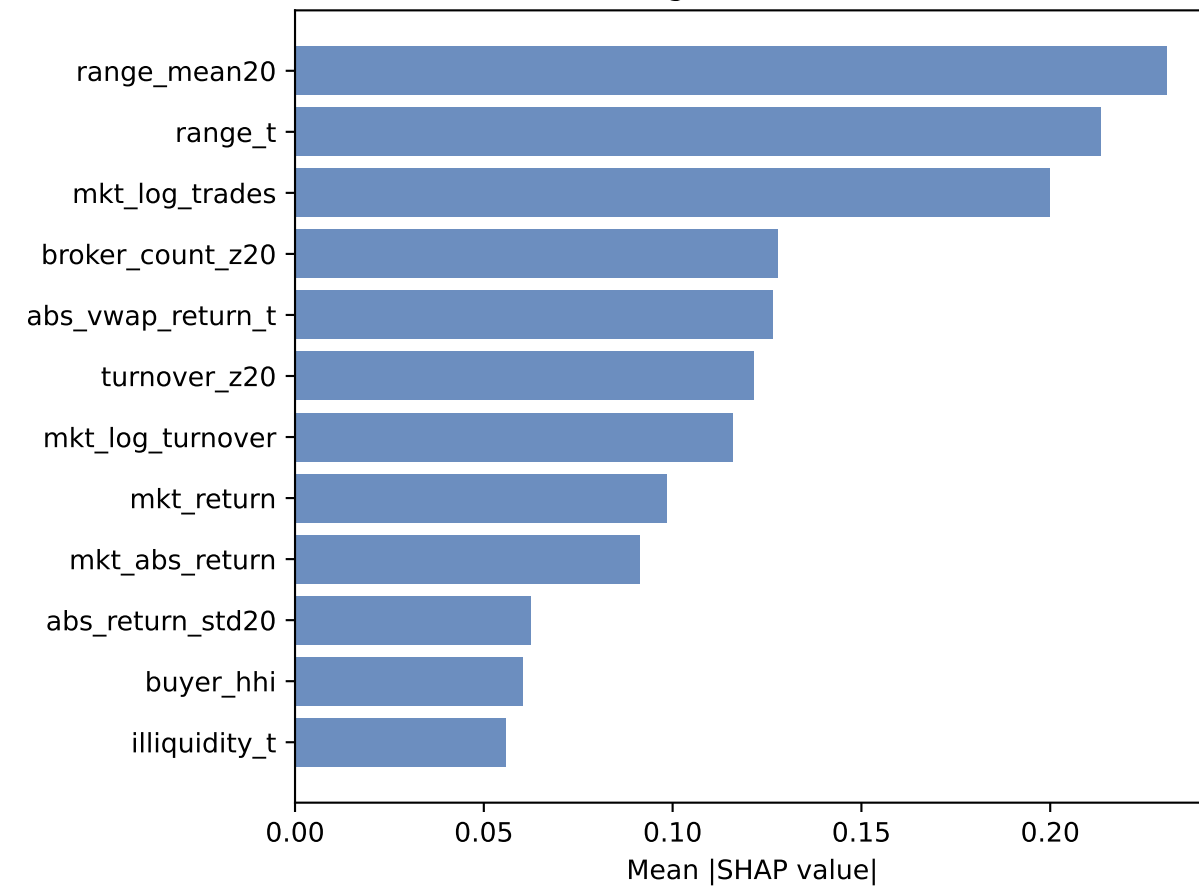
2024 LightGBM TreeSHAP
