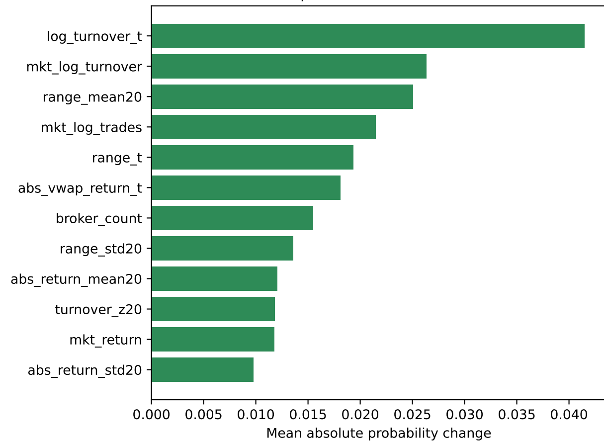
2025 LightGBM TreeSHAP
