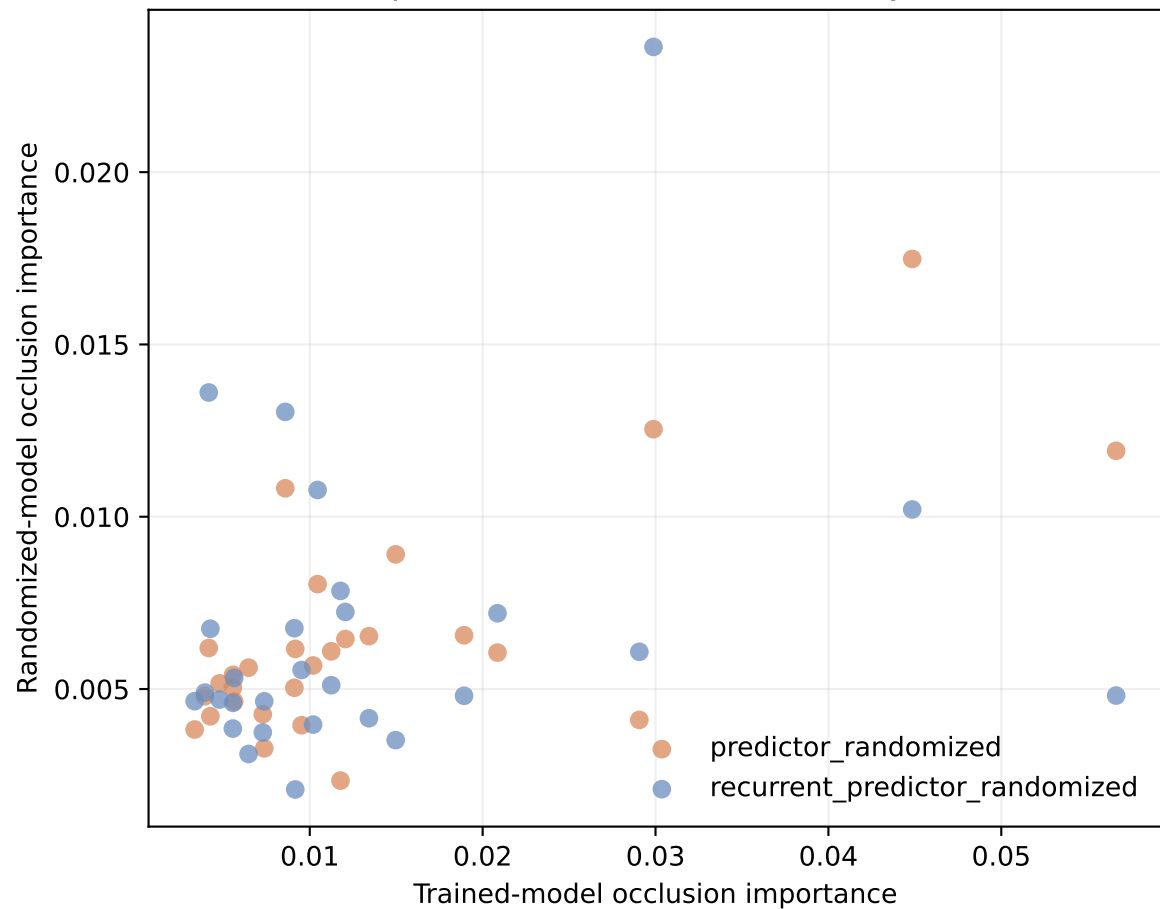
2025 parameter-randomization sanity check
