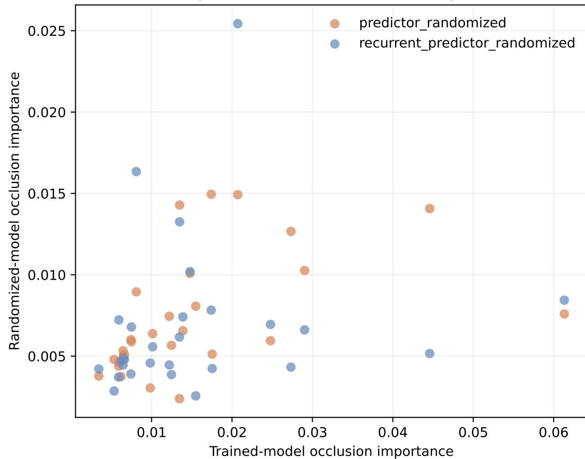
2024 parameter-randomization sanity check
