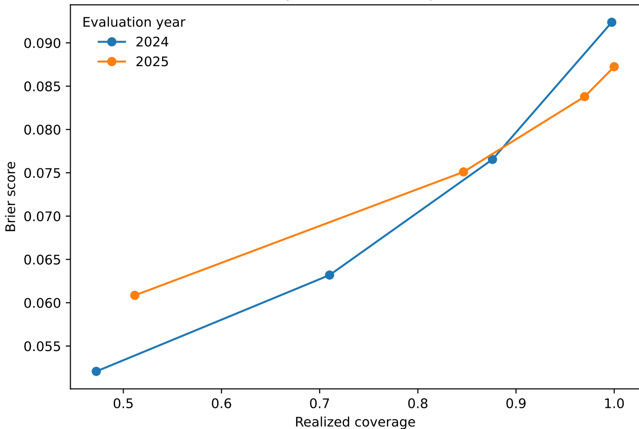
Uncertainty-based selective prediction
