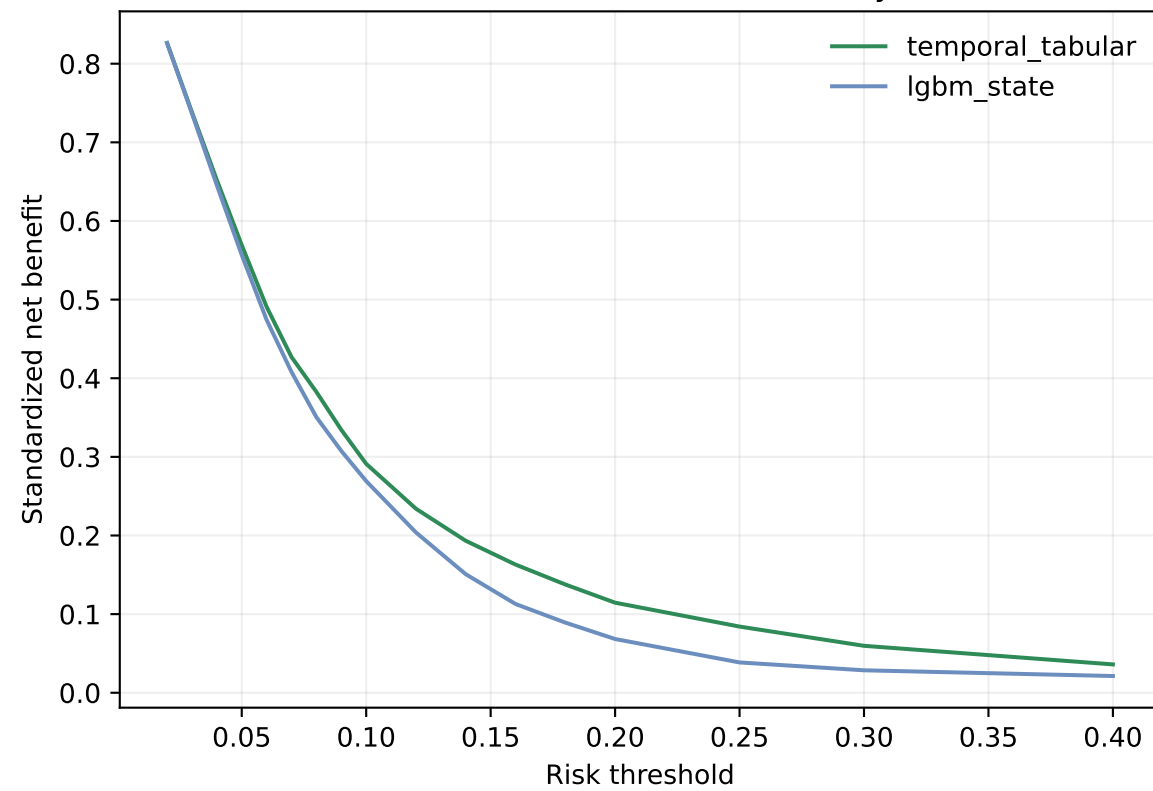
2025: calibrated decision utility
