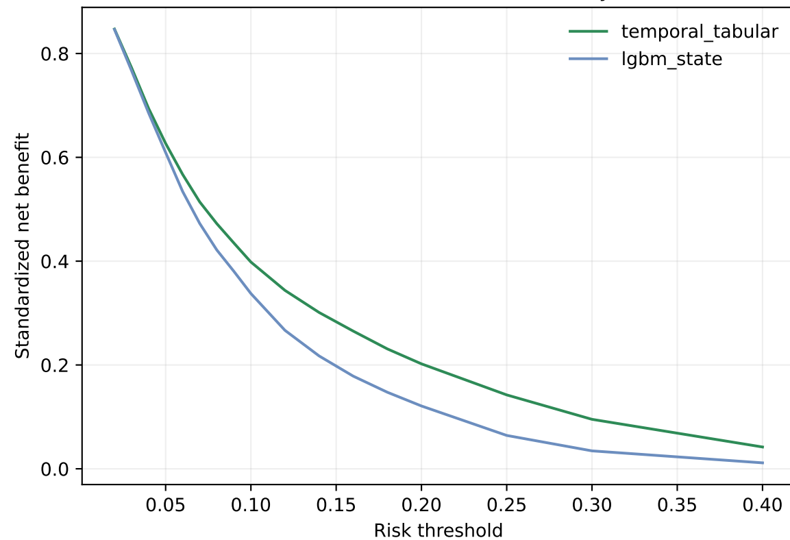
2025: calibrated decision utility
