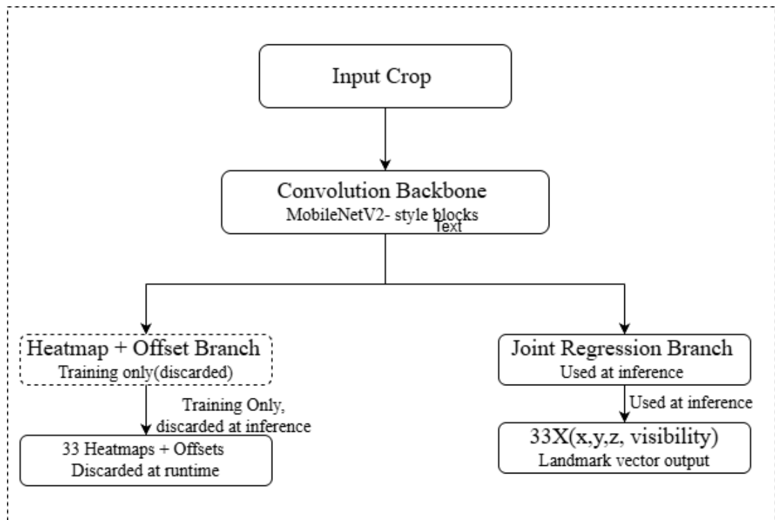
Figure 4-2. Architectural diagram of Mediapipe Pose.
