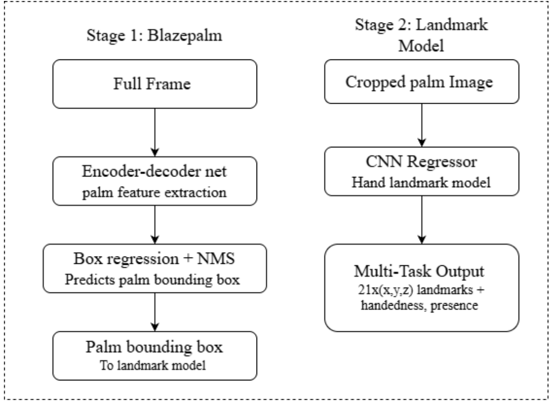
Figure 4-3. Architectural diagram of Mideapipe Hands.
