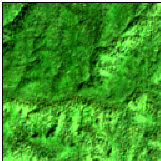
South Asia (49SBT) 1.3 km
