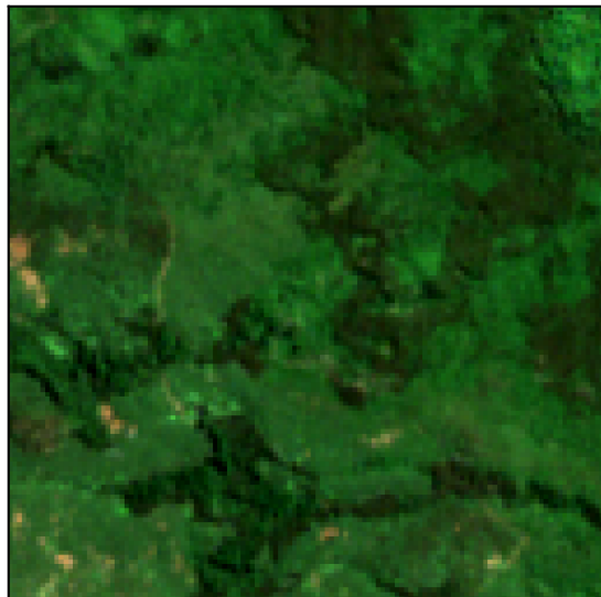
Sentinel-2 (true colour)
