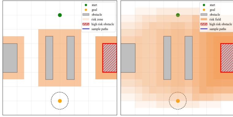
(a) Risk detected by SAM opti- (b) Risk detected by moderate tar- mization get
