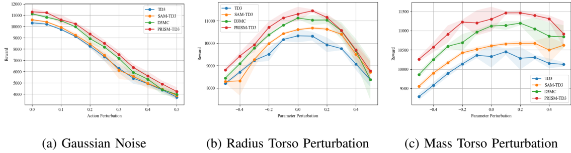
Fig. 3: HalfCheetah-v4
