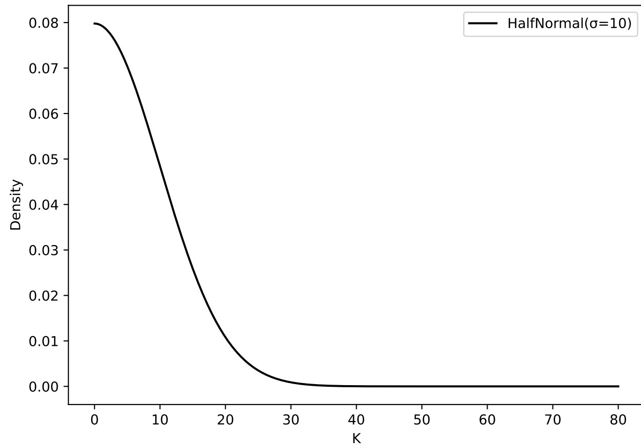
K Priors
