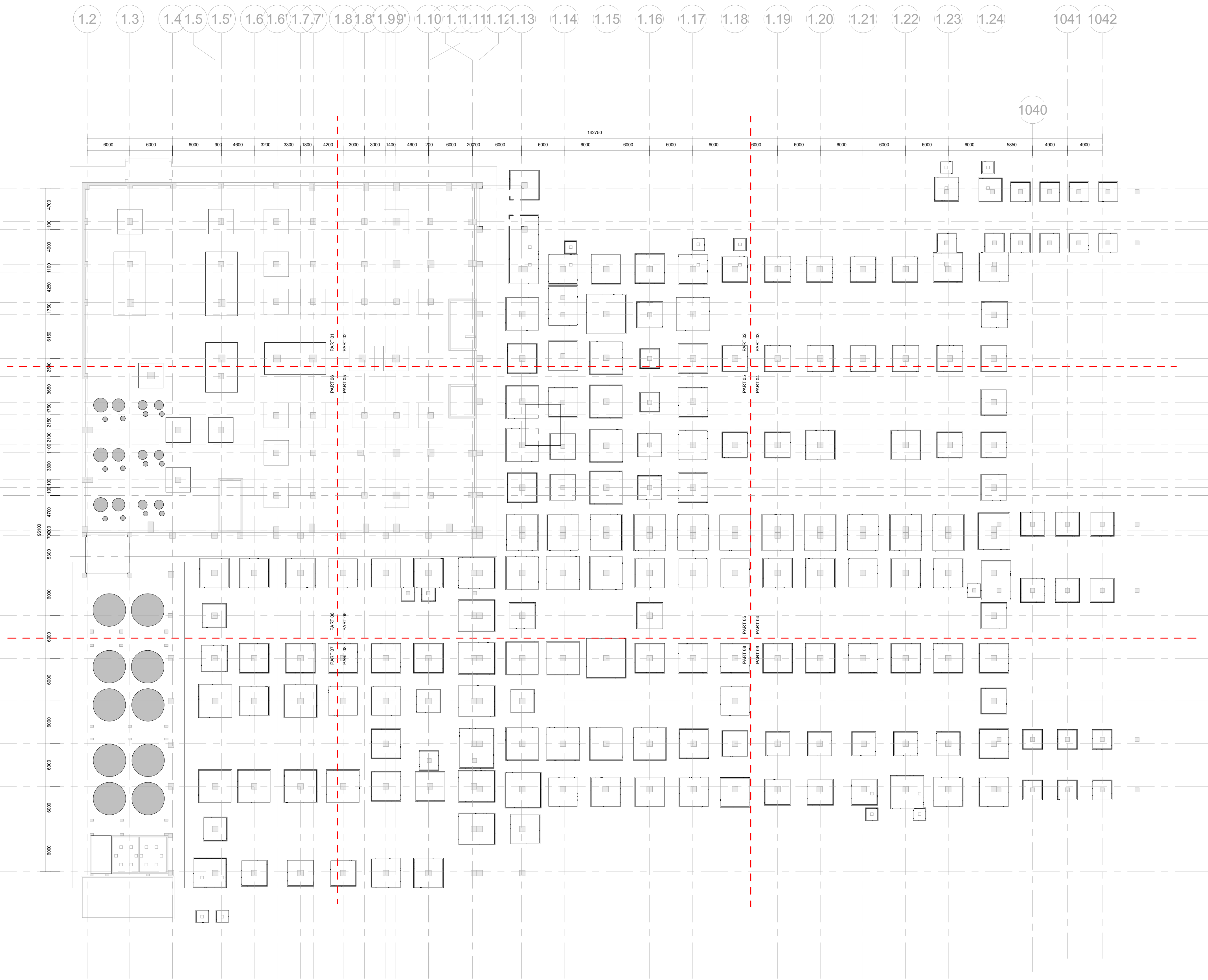
1 FOUNDATION GENERAL ARRANGEMENT OVERALL PLAN 1 : 300
