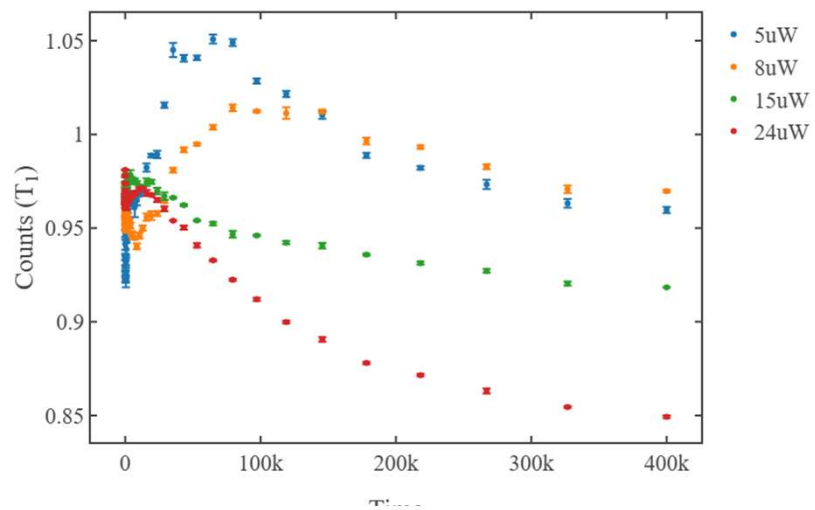
Signal Photon vs Time for 50us Initialization
