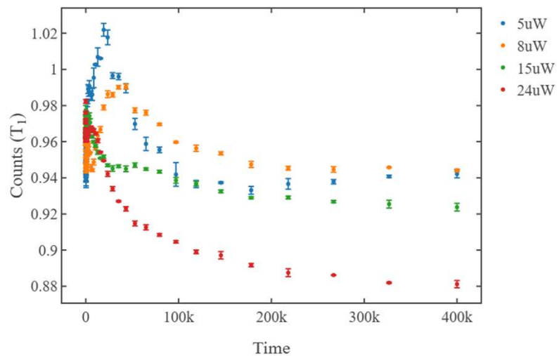
Signal Photon vs Time for 15us Initialization
