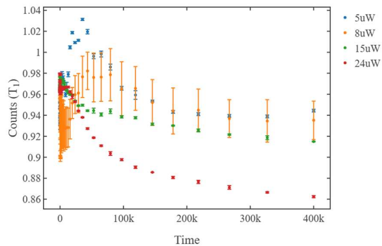
Signal Photon vs Time for 25us Initialization
