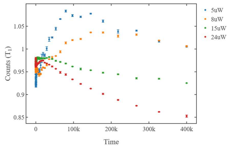
Signal Photon vs Time for 100us Initialization
