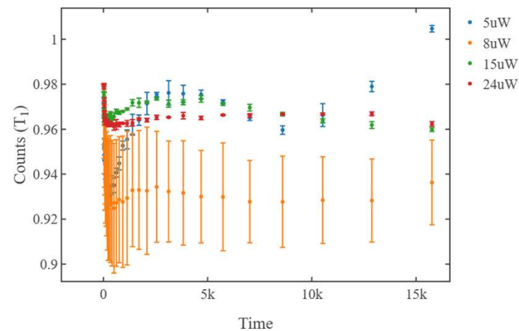
Signal Photon vs Time for 25us Initialization
