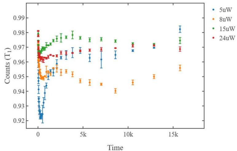
Signal Photon vs Time for 50us Initialization
