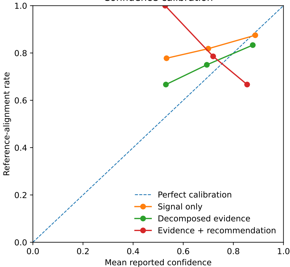
Confidence calibration
