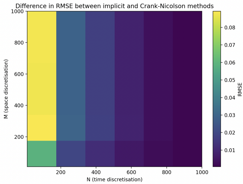
Figure 6: Difference in RMSE between Implicit and Crank-Nicolson Schemes (Implicit-CR)
