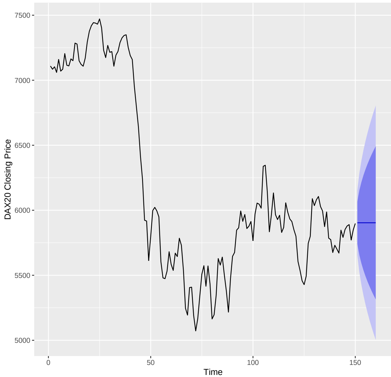
Forecasts from ARIMA(0,1,1)
