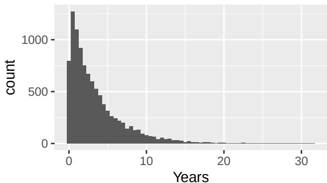
Exponential simulated lifetimes
