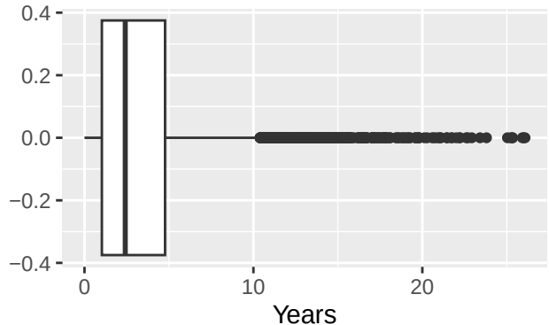
Exponential simulated summary
