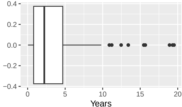
Gamma simulated summary
