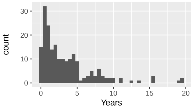
Gamma simulated lifetimes
