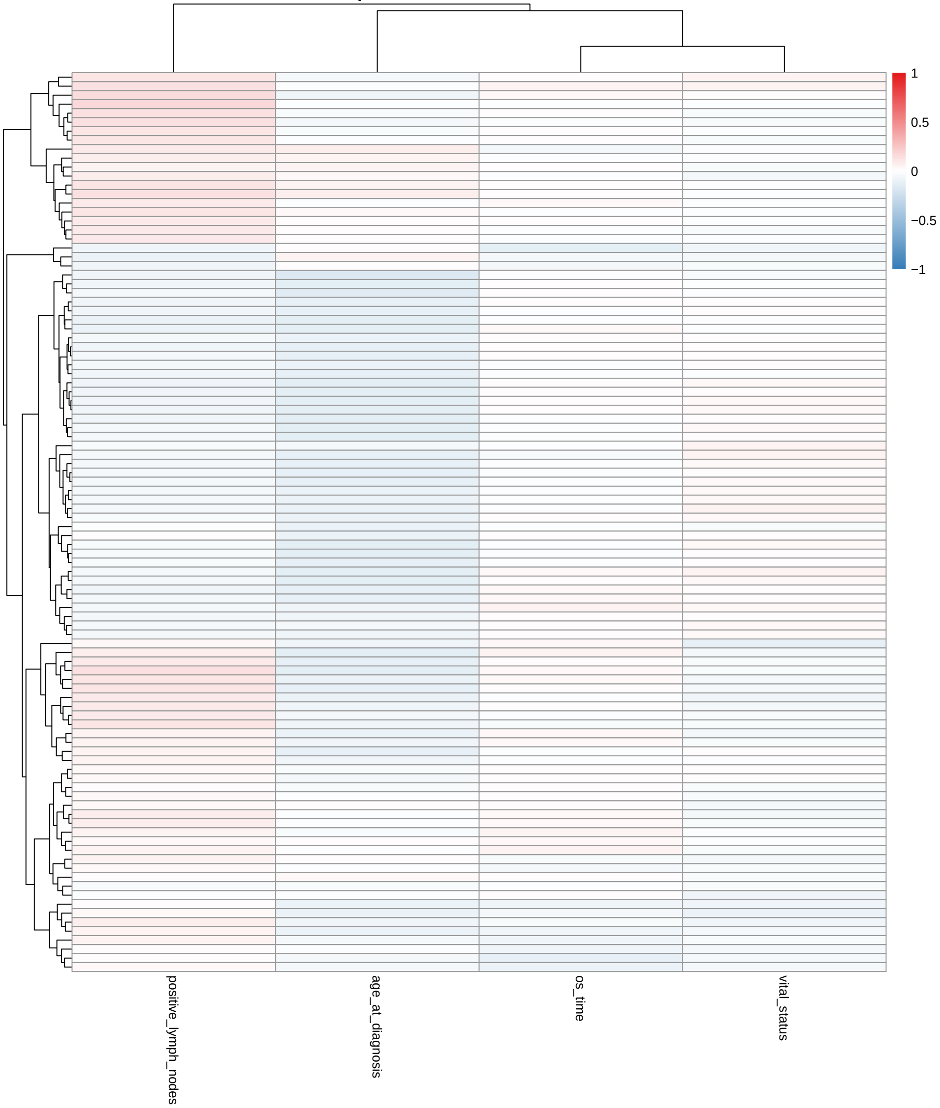
Top 100 DEGs vs Clinical Variables
