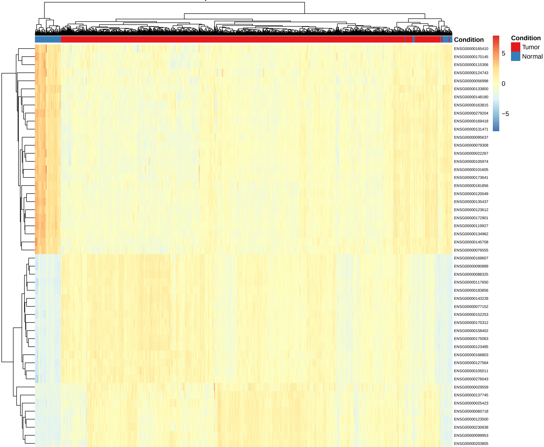
BRCA Top 50 DEGs: Tumor vs Normal
