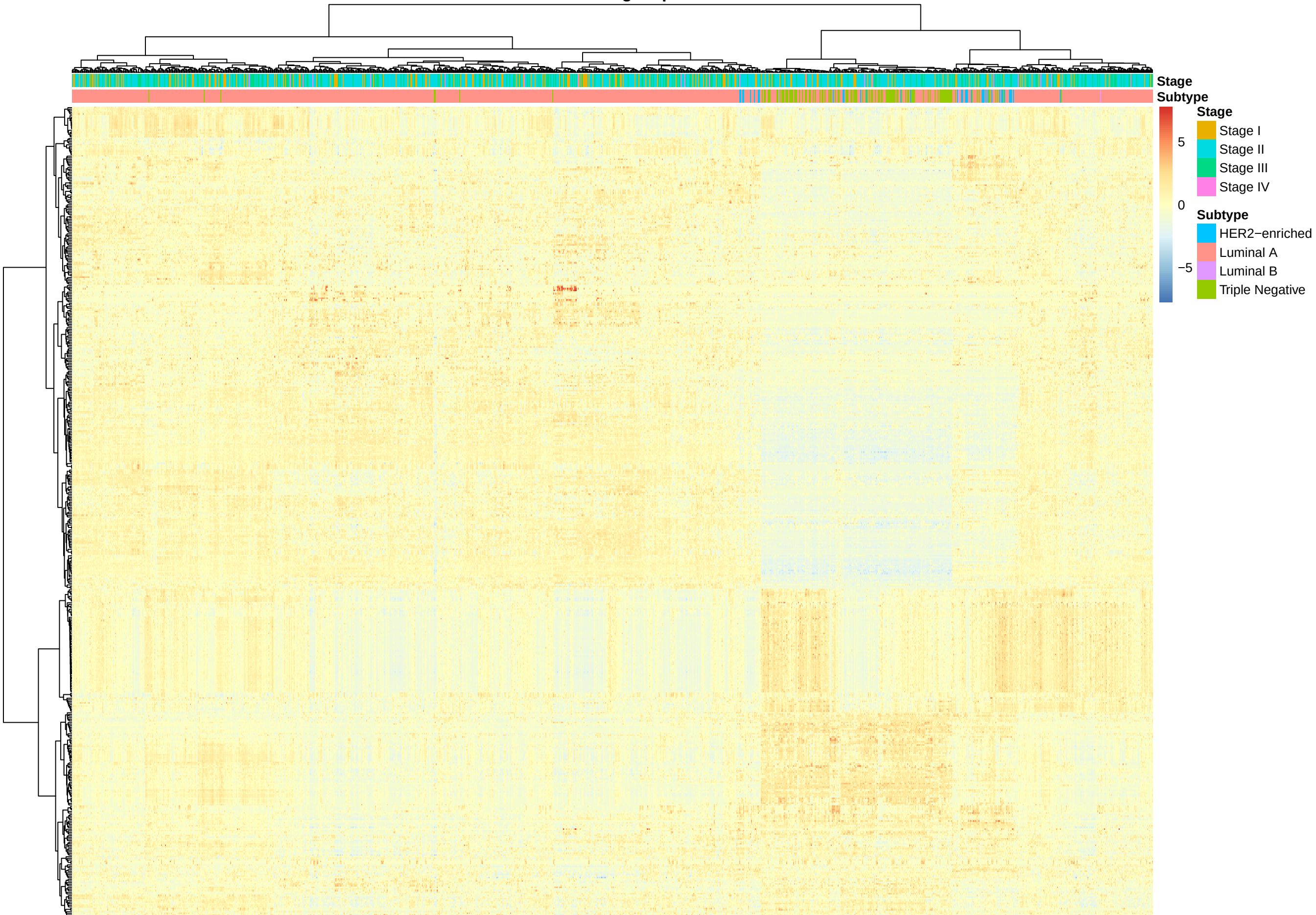
BRCA Hierarchical Clustering: Top 500 Variable Genes
