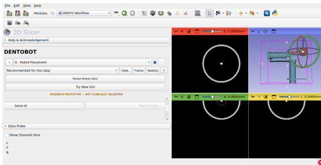
Figure 5. TCP goal widget after orientation nudges and five-joint IK staging. The workbench passed default-off gating, mouse drag, directional/orientation controls and disable cleanup. SHA-256 bab77fd3...d410c.
