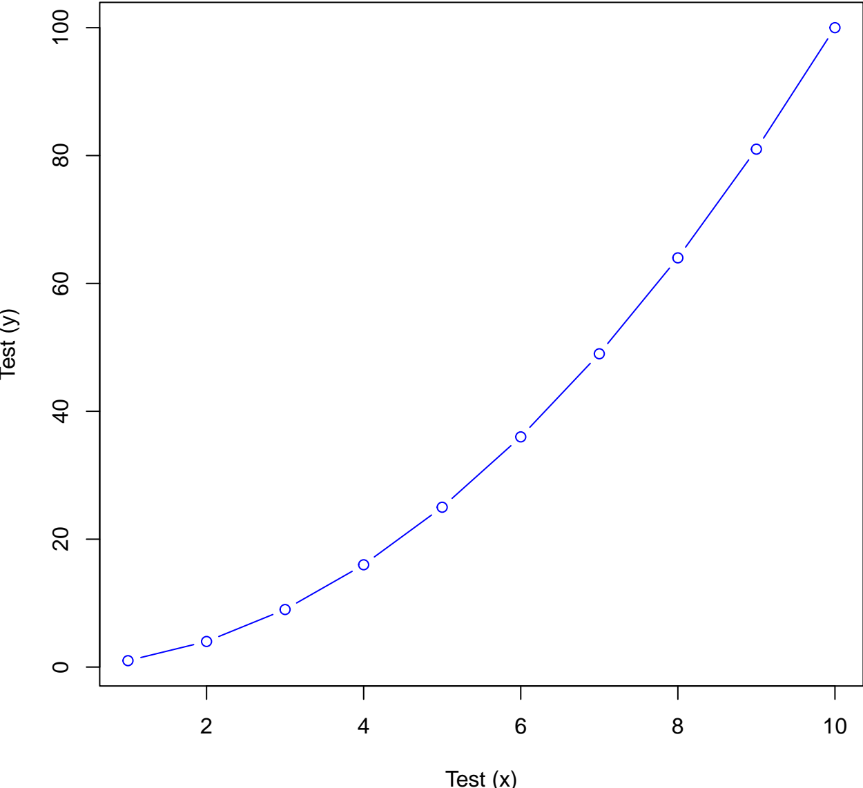
Simple Plot
