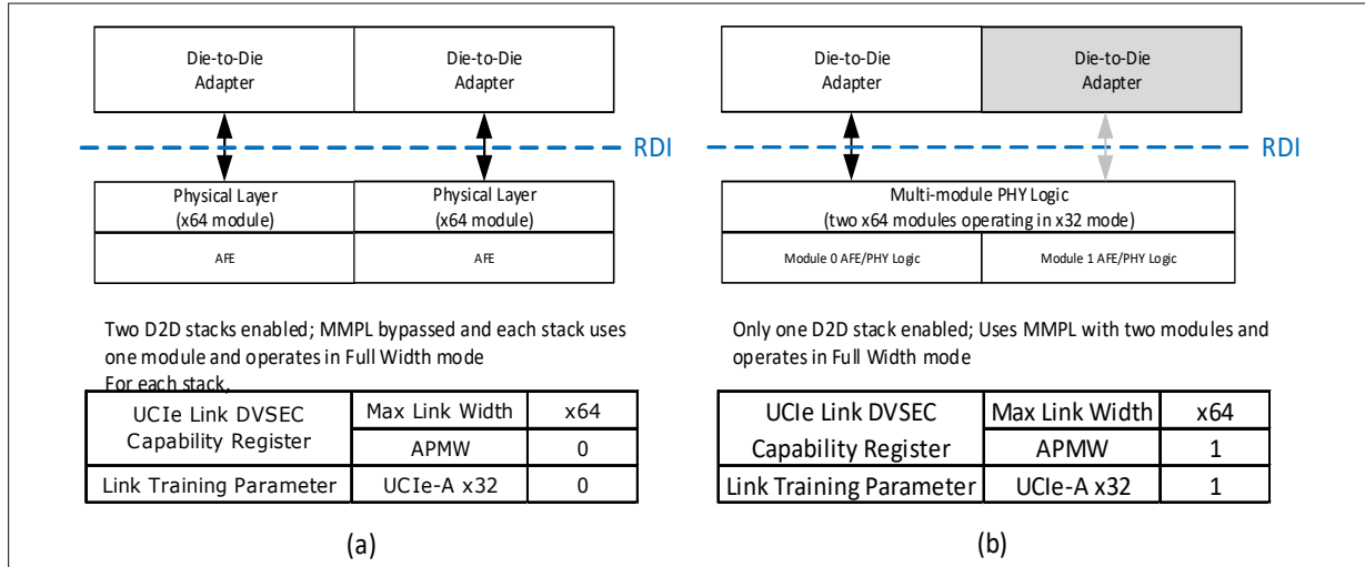
Figure 4-49. Implementation Example Showing Two Different Operating Modes of the Same Hardware Implementation
