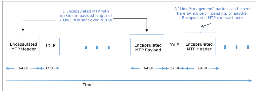
Figure 4-51. Example of Encapsulated MTPs Transmitted on Sideband Link without Sideband PMO
