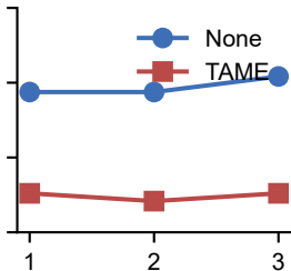
S3 Retrieval
