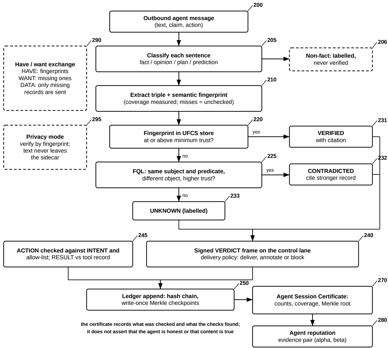
FIG. 2 — Verified Agent Transport — Claim Verification, Intent Binding and Session Certification
