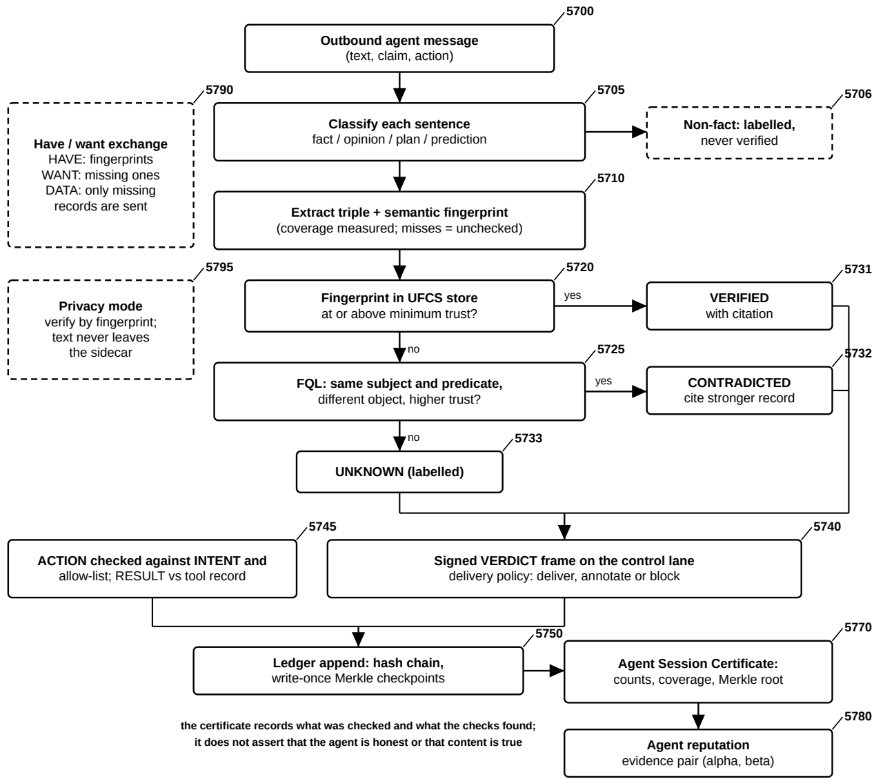
FIG. 57 — Verified Agent Transport — Claim Verification, Intent Binding and Session Certification
