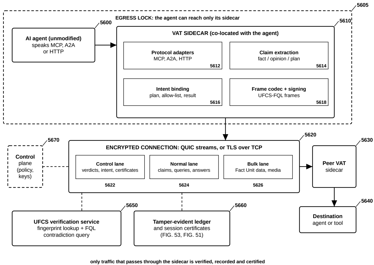
FIG. 56 — Verified Agent Transport — Sidecar, Egress Lock and Lanes over an Encrypted Connection
