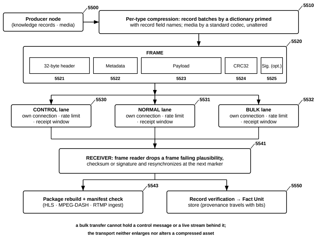
FIG. 24 — Hybrid Transport — Framed UFCS-FQL Messages on Priority Lanes over TCP/IP (extends FIG. 17)
