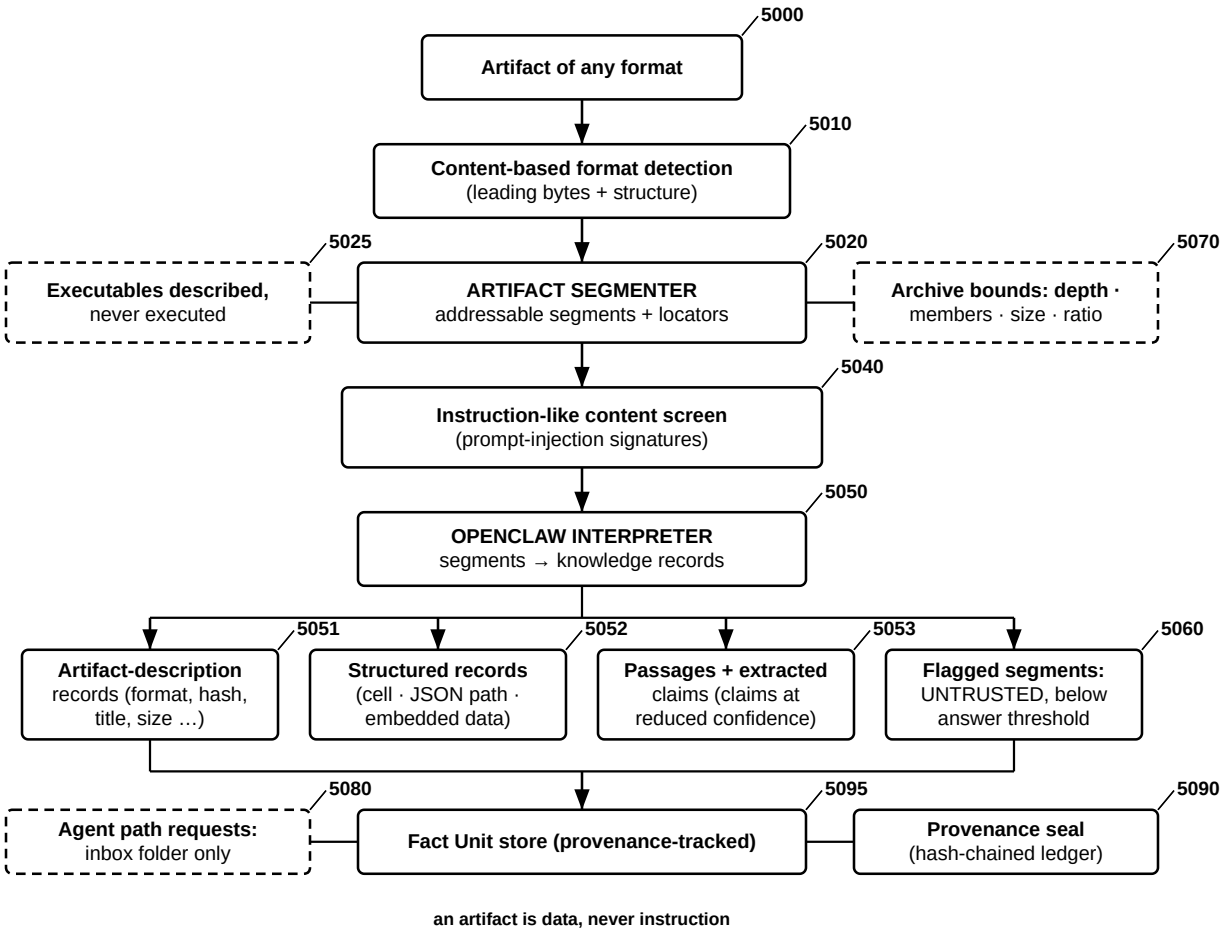
FIG. 19 — Open Claw Ingestion — Artifact Segmenter and OpenClaw Interpreter
