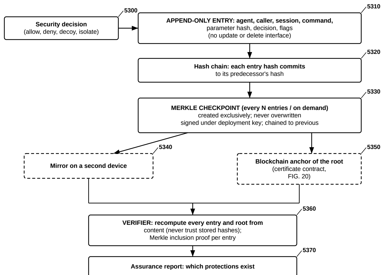
FIG. 22 — Tamper-Evident Security Record — Hash Chain, Write-Once Merkle Checkpoints, Mirror and Anchor
