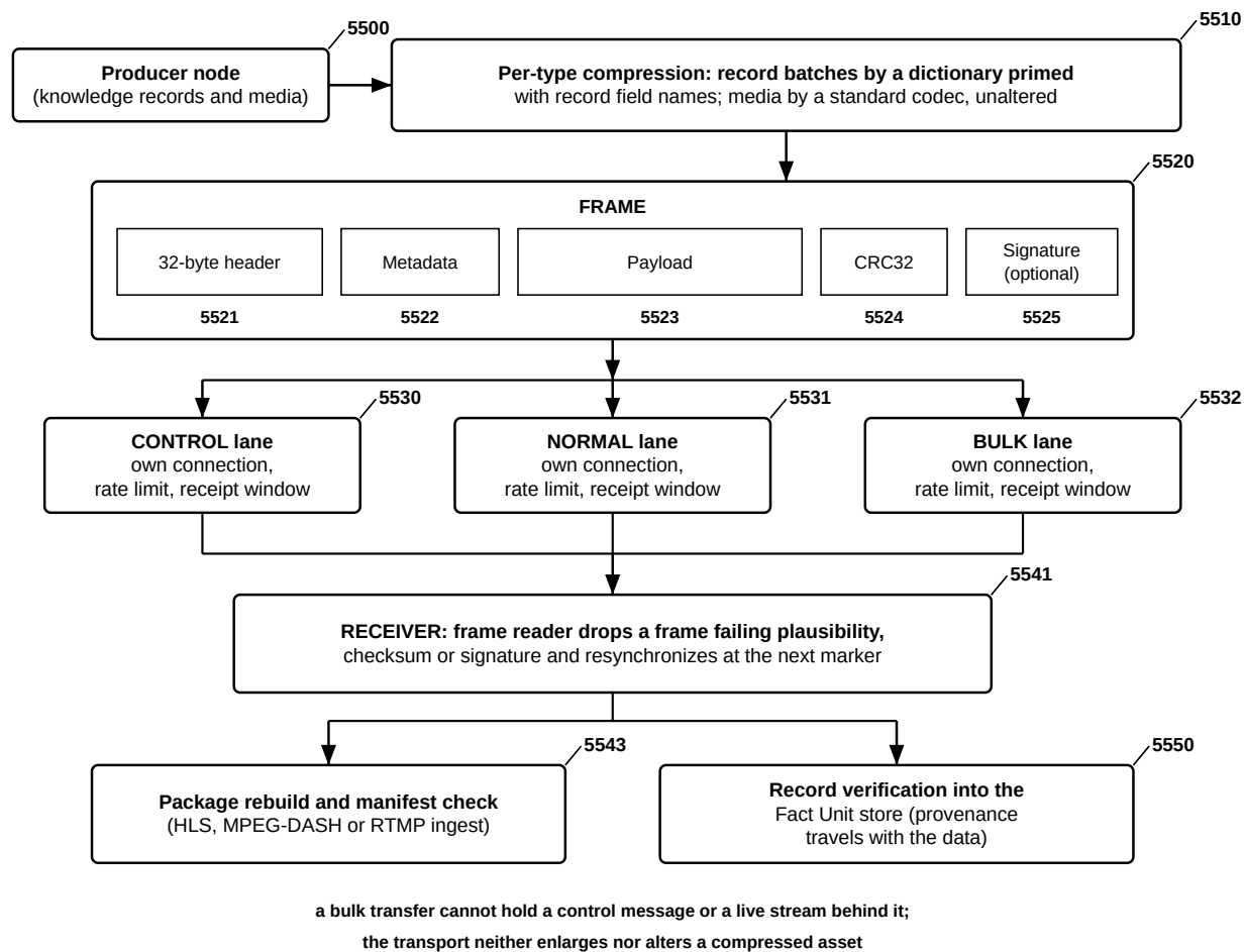
FIG. 24 — Hybrid Transport — Framed Messages on Priority Lanes over TCP/IP (extends FIG. 17)
