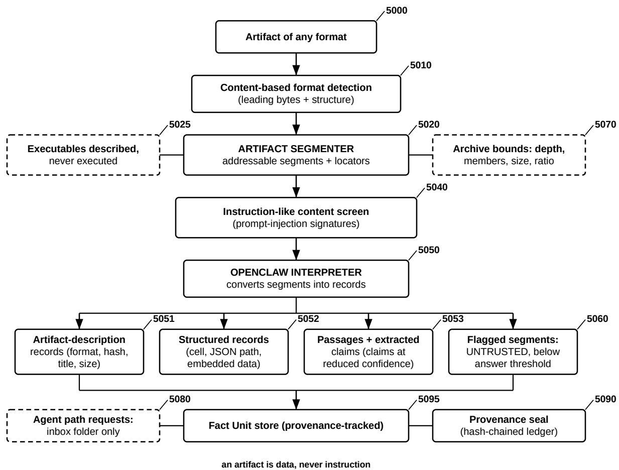
FIG. 19 — Open Claw Ingestion — Artifact Segmenter and OpenClaw Interpreter
