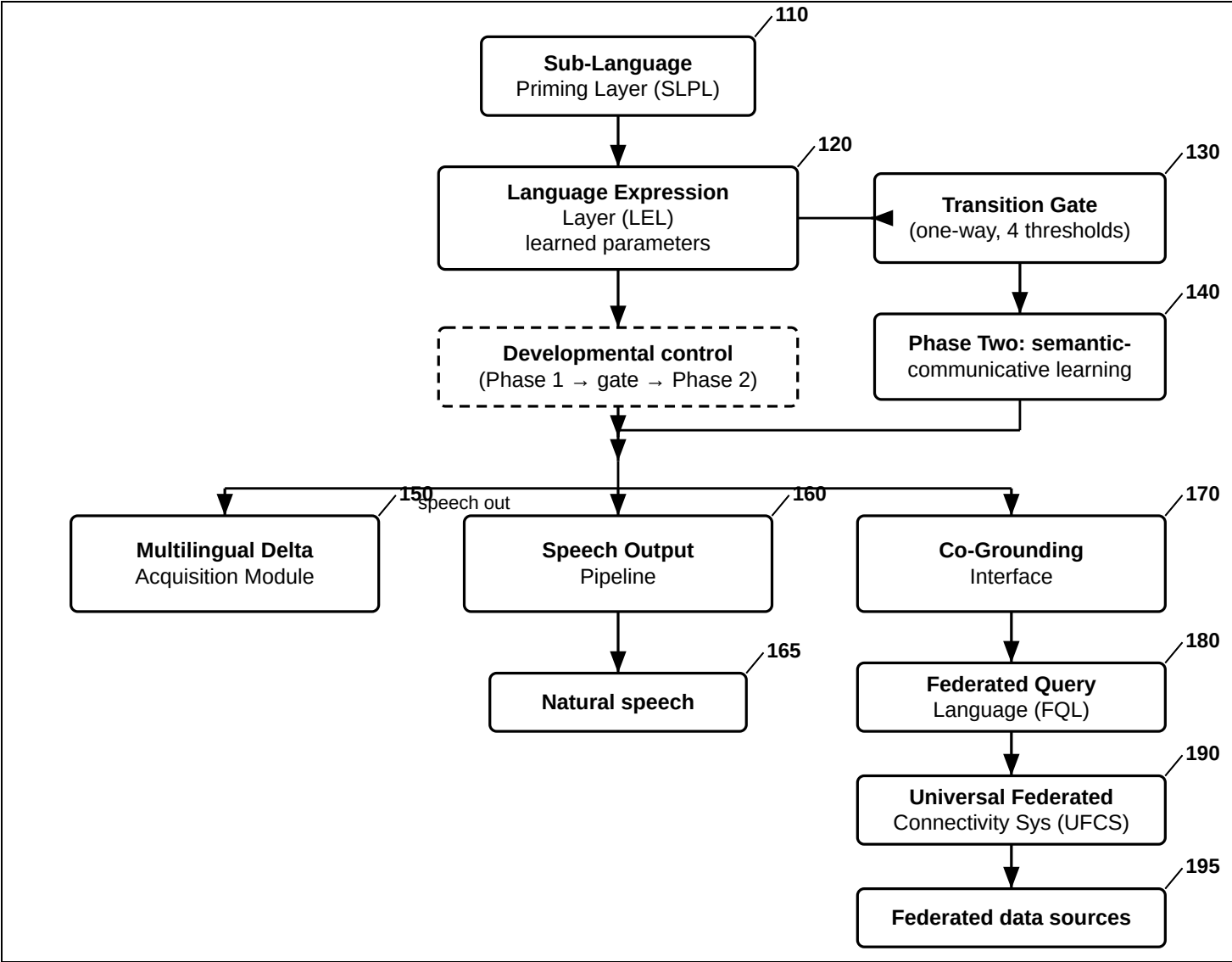
FIG. 1 — QueryBook LEL — Overall System Architecture
