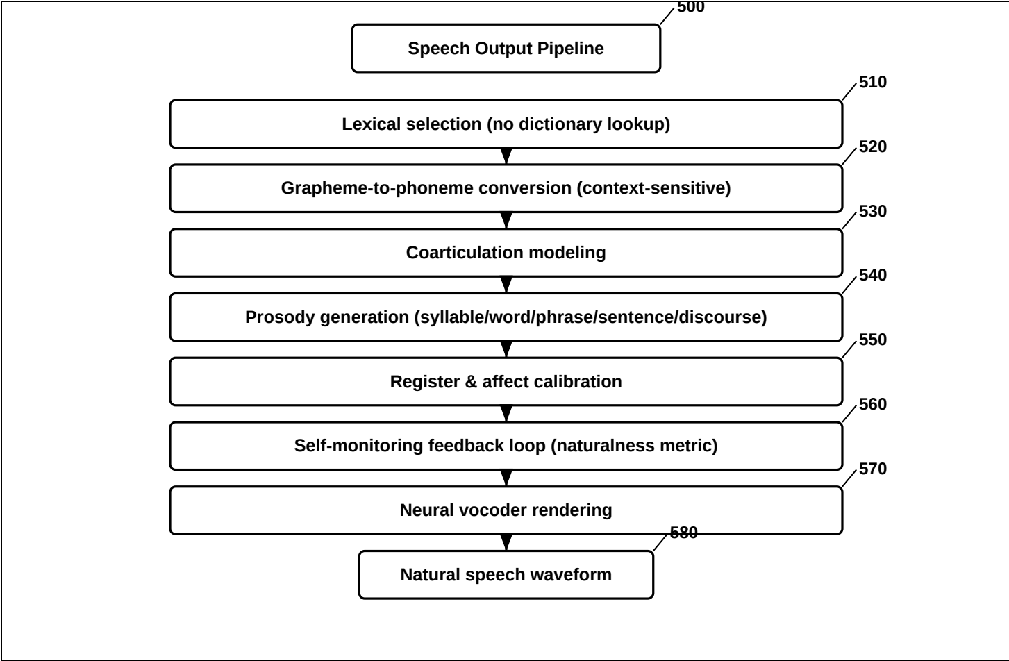
FIG. 5 — Speech Output Pipeline (Seven Learned Stages)
