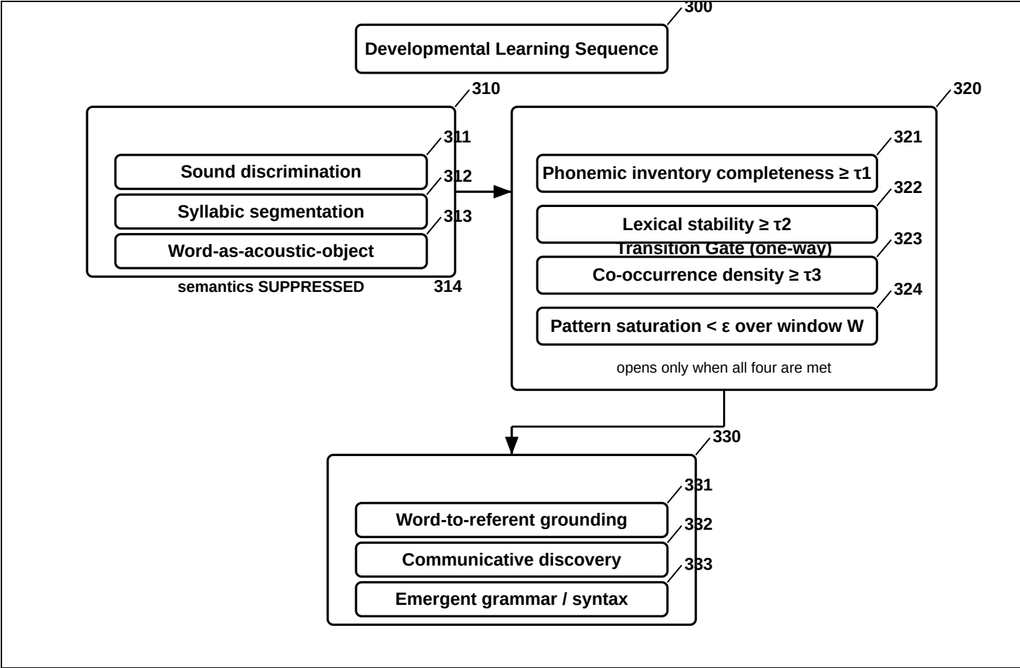
FIG. 3 — Developmental Learning Sequence and One-Way Transition Gate
