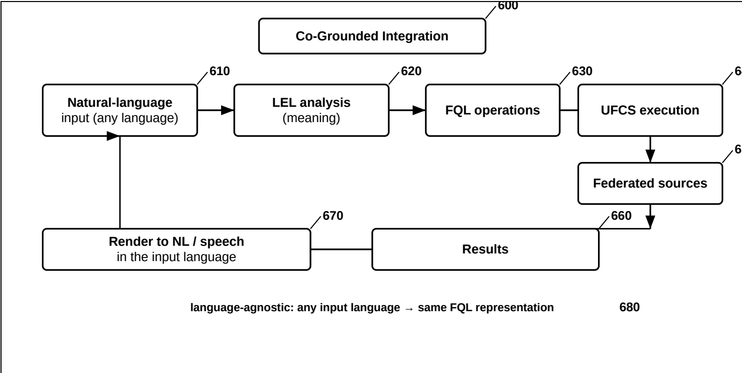
FIG. 6 — Co-Grounded Integration with FQL and UFCS
