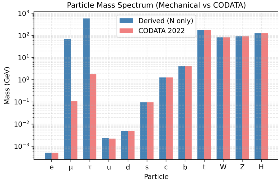
Figure 10: Quantized mass hierarchy derived from harmonic modes.
