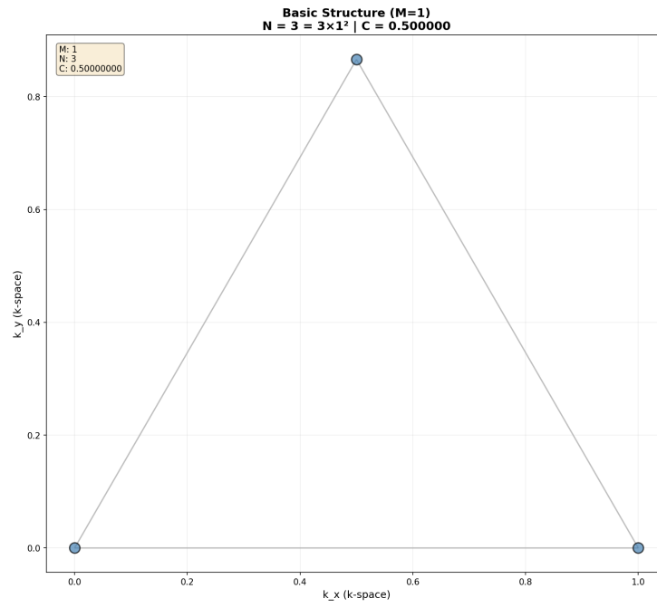
Figure 2: Minimal 3-node primordial triangular bond. C = 0.500000
