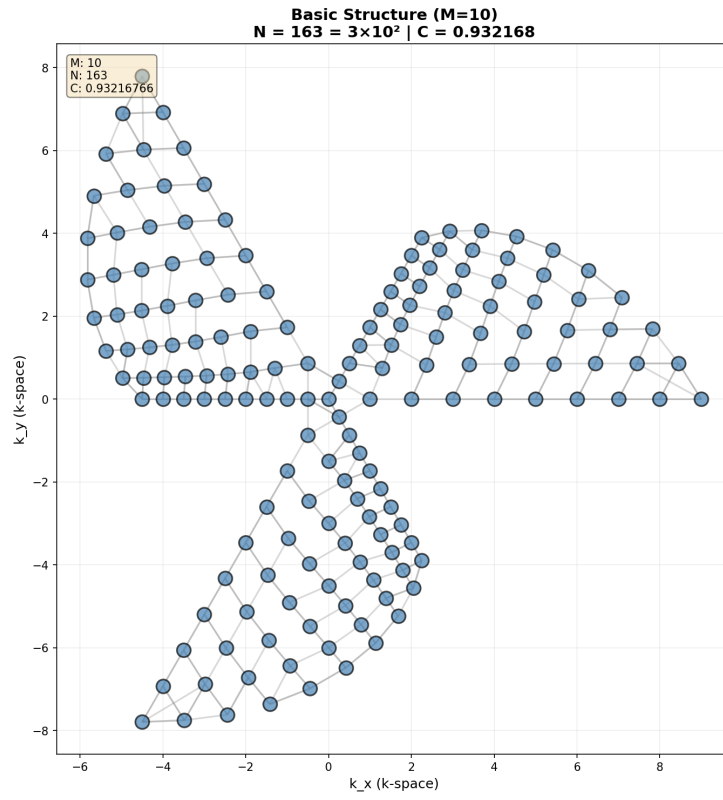
Figure 8: Near-continuum manifold approximation. C = 0.932168
