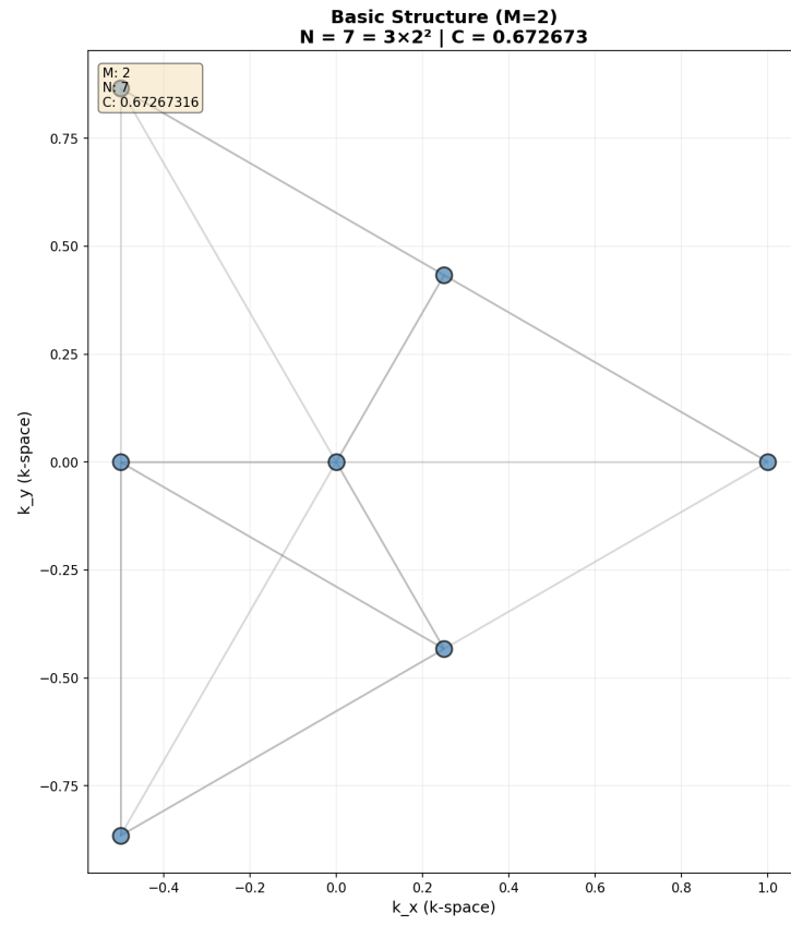
Figure 3: First-order expansion showing 7 active nodes. C = 0.672673
