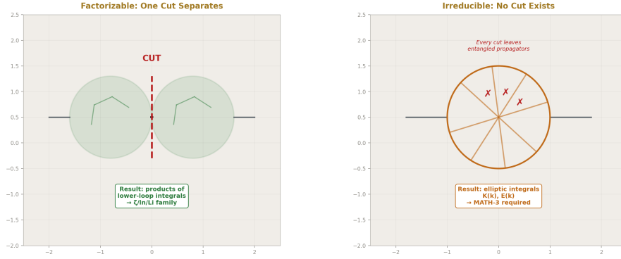
Figure 6: Fig. 7: If one cut separates the graph, integrals factorize into \zeta/\ln/\text{Li} . If no cut exists, elliptic integrals appear.
