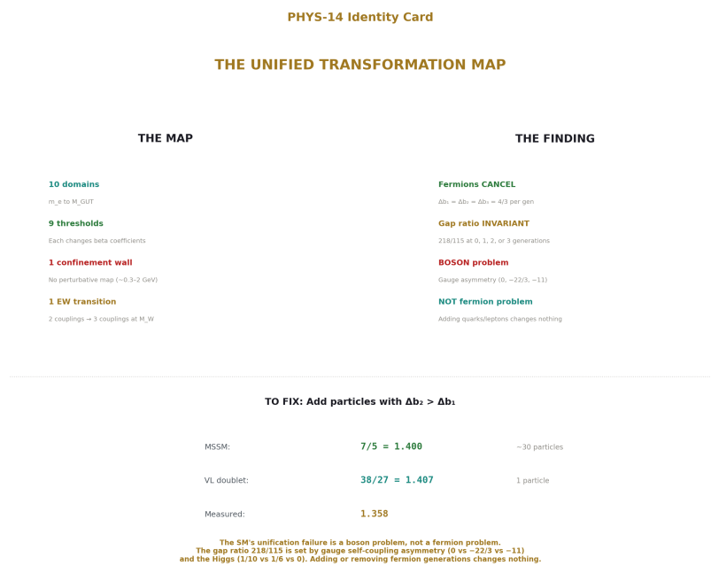
Figure 8: Fig. 8: 10 domains, fermion cancellation ( \Delta b_1=\Delta b_2=\Delta b_3=4/3 ), boson problem (gauge asymmetry sets 218/115), fix requires asymmetric BSM content (VL doublet or MSSM).
