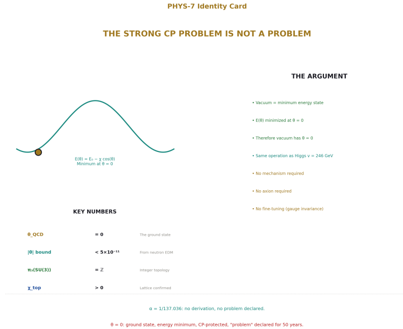
Figure 8: Fig. 8: \theta=0 is the ground state of an integer-topological system — the energy functional, the integer topology, the double standard, and no mechanism required.
