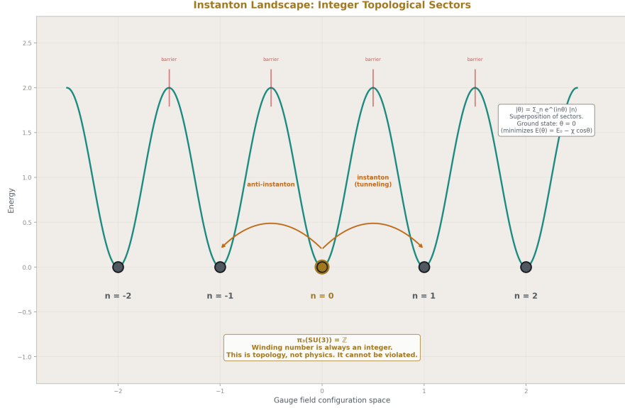
Figure 3: Fig. 3: Periodic energy barriers between integer topological sectors n \in \mathbb{Z} . Instantons tunnel between adjacent sectors. The ground state at n=0 is the minimum of the cosine potential.
