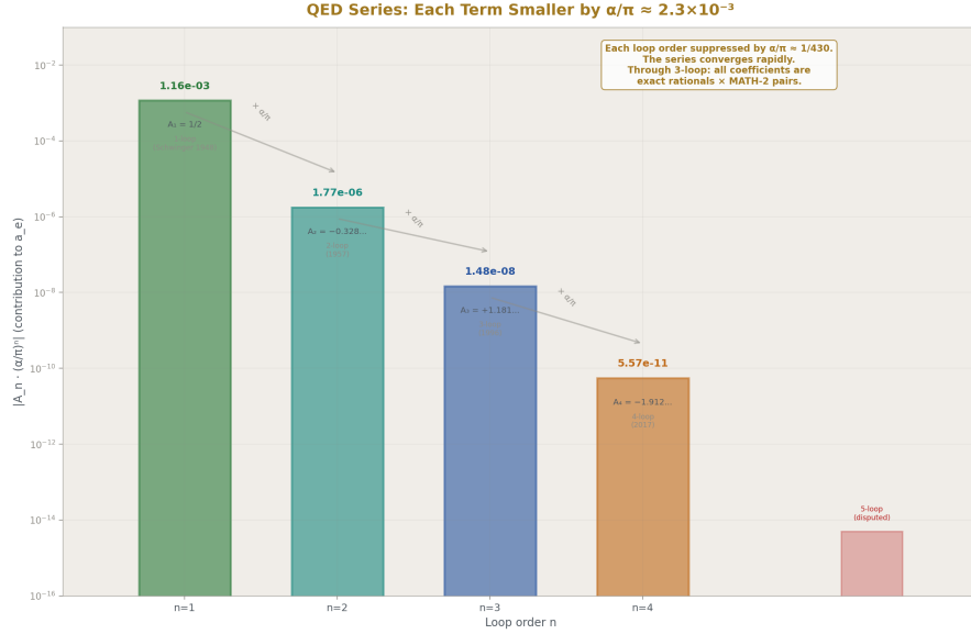
Figure 1: Fig. 7: Each QED loop order is suppressed by \alpha/\pi \approx 1/430 — the series converges rapidly and through 3-loop every coefficient is exact rationals times MATH-2 pairs.
