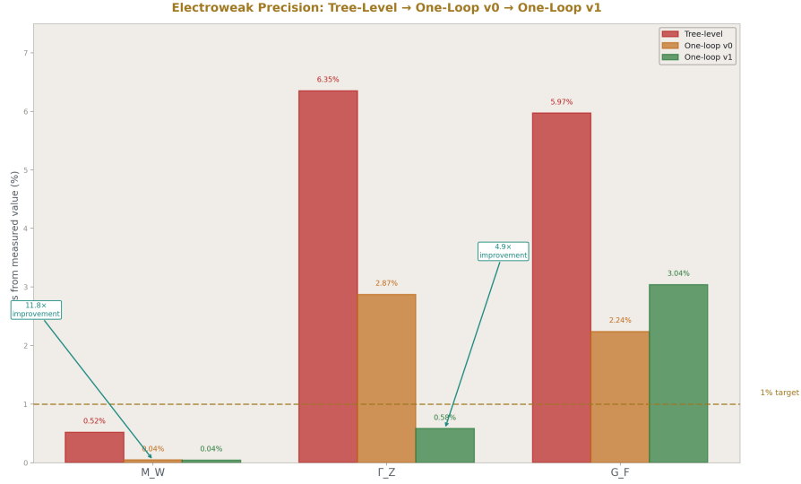
Figure 3: Fig. 7: M_W improves 11.8 \times (tree \rightarrow v0), \Gamma_Z improves 4.9 \times (v0 \rightarrow v1) — the bars show each correction closing the gap to the measured values.
