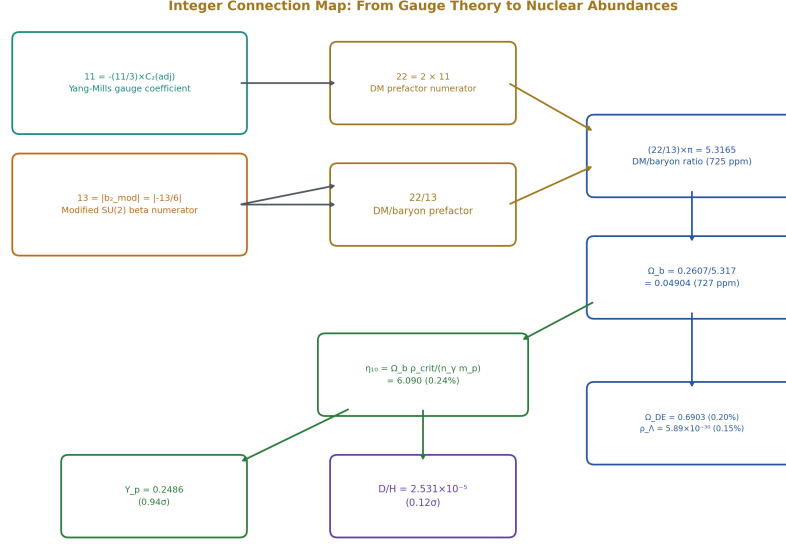
Figure 5: Fig. 6: The integers 11 and 13 flow through (22/13) \pi to DM/baryon, through \Omega_b and \eta to Y_p and D/H — every node carries a computed value.
