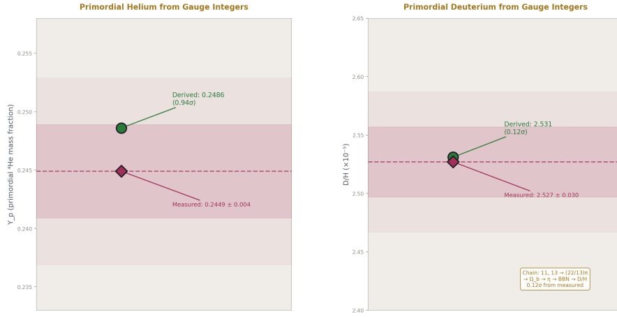
Figure 4: Fig. 5: Primordial helium (0.94 \sigma ) and deuterium (0.12 \sigma ) predicted from gauge integers — both within measurement uncertainties.
