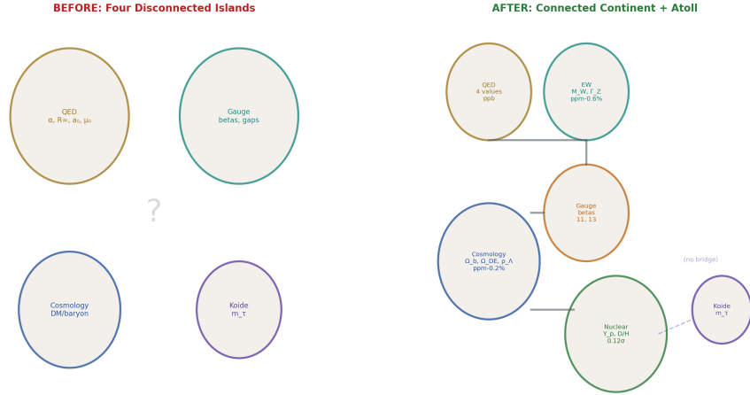
Figure 7: Fig. 4: Four disconnected islands merge into one connected continent through ten bridge derivations — only Koide remains as a floating atoll.
