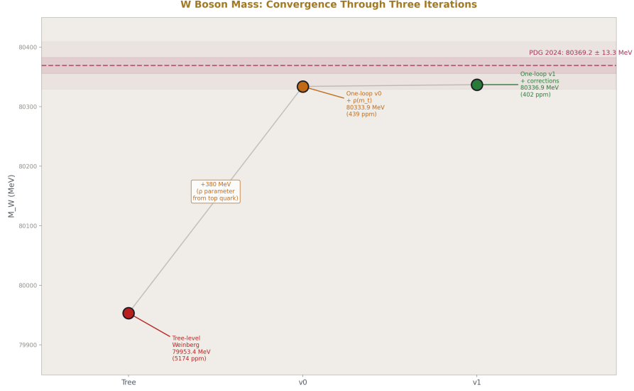
Figure 2: Fig. 2: M_W converges from 79953 (tree) to 80337 (one-loop v_1 ), approaching the measured 80369 — the \rho parameter adds 380 MeV from the top quark.
