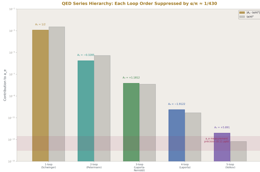
Figure 2: Fig. 2: Each QED loop order is suppressed by \alpha/\pi \approx 1/430 — the 5-loop term sits at the measurement precision.
