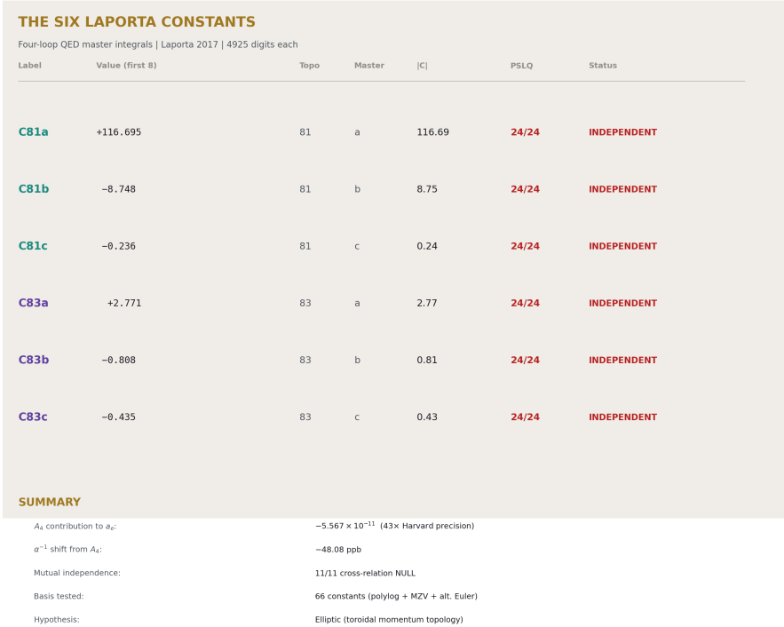
Figure 1: Fig. 8: Identity card. Six constants, two topologies, 4925 digits each, 24/24 PSLQ null, 43 \times Harvard precision, 48 ppb \alpha shift, 11/11 mutually independent.
