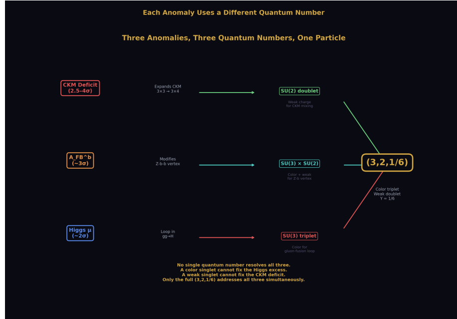
Figure 1: Fig. 1: CKM deficit needs SU(2) (weak doublet for CKM mixing), A_{FB}^b needs SU(3) \times SU(2) (color+weak for Z-b vertex), Higgs \mu needs SU(3) (color for gg \rightarrow H loop). Only (3, 2, 1/6) has all three.
