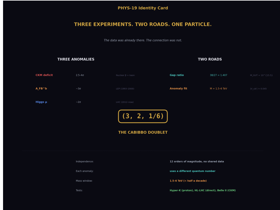
Figure 7: Fig. 8: Three experiments (LEP, LHC, nuclear/kaon) across three decades produced three anomalies resolved by one particle identified independently by gap ratio arithmetic. The data was there. The connection was not.
