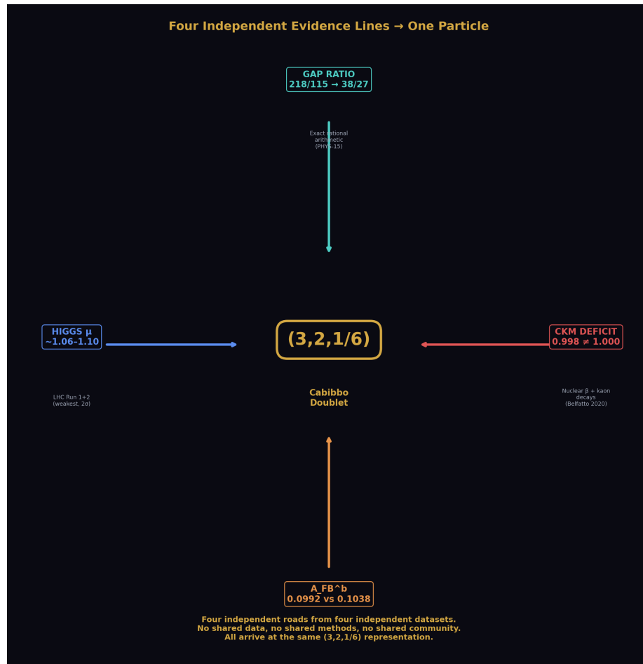
Figure 4: Fig. 5: Gap ratio (exact arithmetic), CKM deficit (nuclear \beta ), A_{FB}^b (LEP), Higgs \mu (LHC) — four independent arrows from four independent datasets, all converging on (3,2,1/6).
