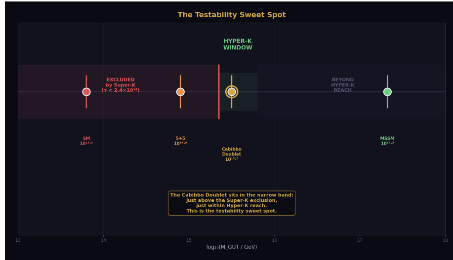
Figure 3: Fig. 2: The Cabibbo Doublet at M_{\text{GUT}} = 10^{15.5} sits in a narrow testability band — just above the Super-K exclusion, just within Hyper-K reach. The MSSM at 10^{17.3} is far beyond any planned experiment.
