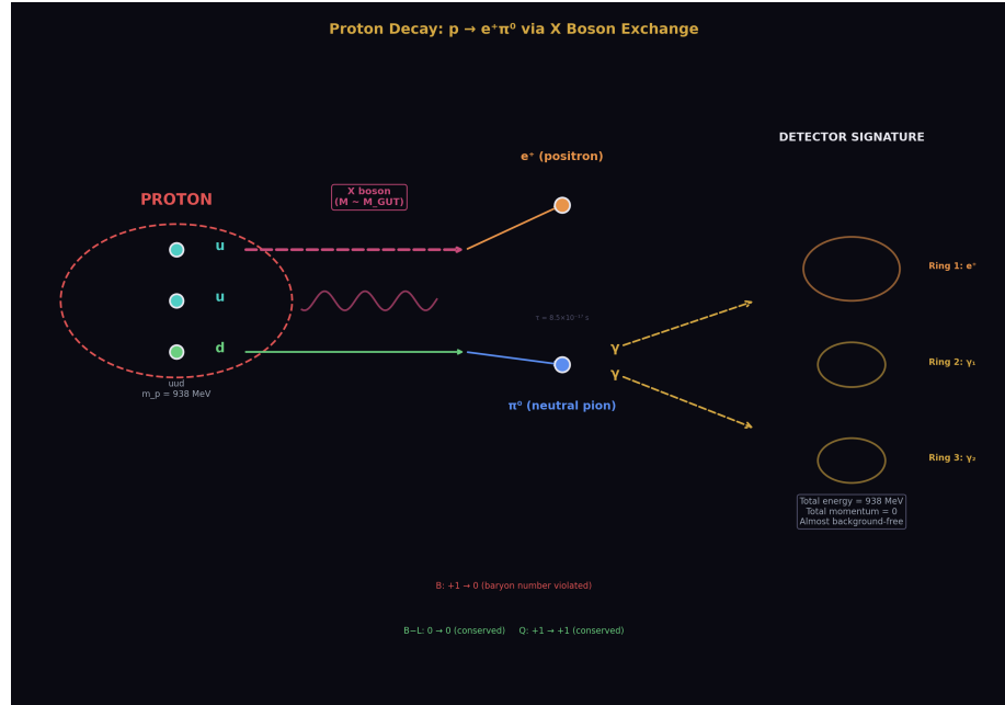
Figure 1: Fig. 6: Proton (uud) exchanges an X boson at M_{\text{GUT}} — one quark converts to positron, remaining quarks form \pi^0 \rightarrow \gamma\gamma . Three Cherenkov rings at 938 MeV total energy, zero momentum, almost background-free.
