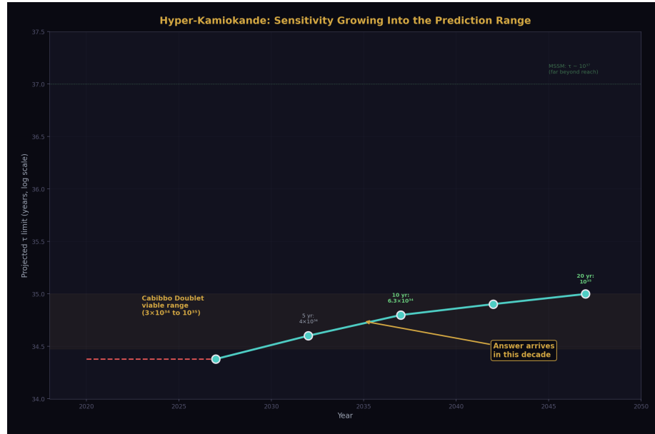
Figure 5: Fig. 3: Hyper-K projected proton decay limit improves from 2.4 \times 10^{34} yr (Super-K legacy) to 10^{35} yr over 20 years. The Cabibbo Doublet viable range ( 3 \times 10^{34} to 10^{35} ) is fully covered by ~2047.
