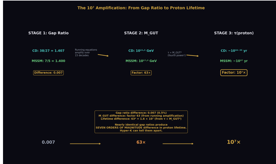
Figure 6: Fig. 5: Gap ratio difference 0.007 \rightarrow M_{GUT} factor 63 (running amplification) \rightarrow lifetime factor 10^7 (fourth power). Nearly identical gap ratios produce seven orders of magnitude separation in proton lifetime.
