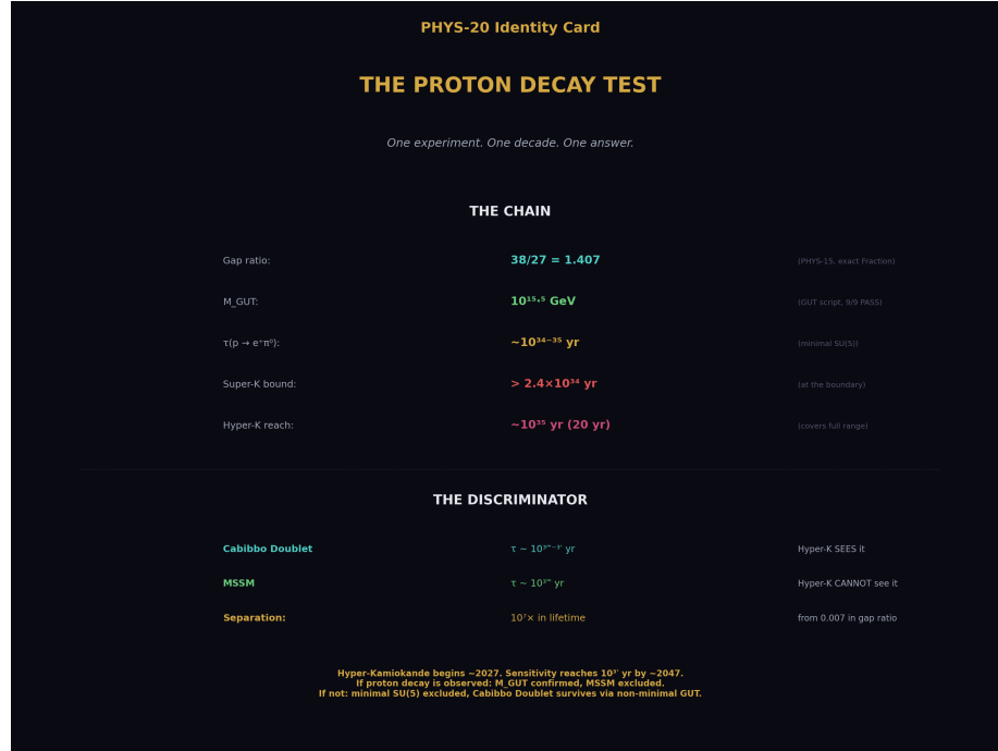
Figure 8: Fig. 8: Gap ratio 38/27 \rightarrow M_{\text{GUT}} = 10^{15.5} \rightarrow \tau \sim 10^{34-35} yr. Cabibbo Doublet and MSSM separated by 10^7 in lifetime despite 0.007 in gap ratio. Hyper-K 2027–2047 covers the full range.
