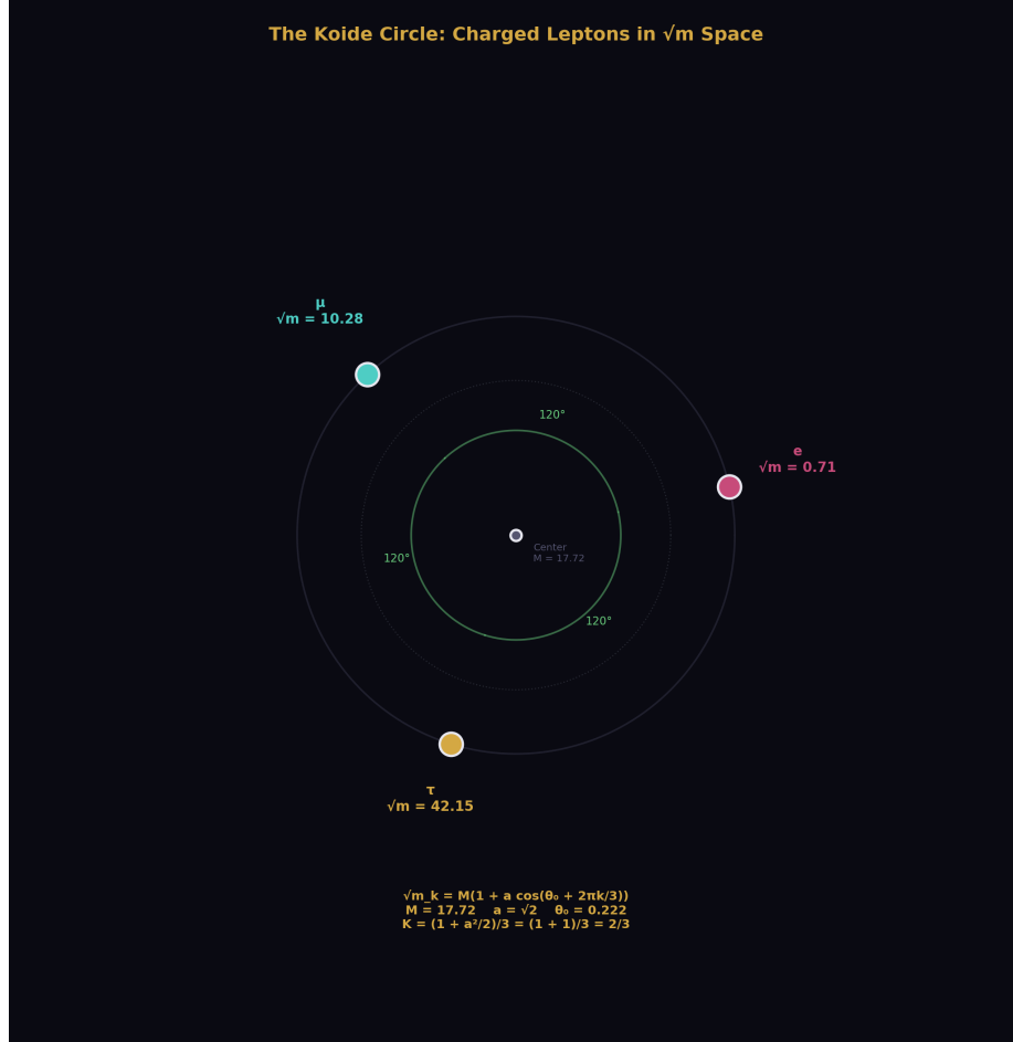
Figure 1: Fig. 3: \sqrt{m}_e, \sqrt{m}_\mu, \sqrt{m}_\tau placed on a circle at 120^\circ intervals in \sqrt{m} space. M = 17.72 , a = \sqrt{2} , \theta_0 = 0.222 . The parametrization K = (1+a^2/2)/3 = 2/3 when a^2 = 2 .
