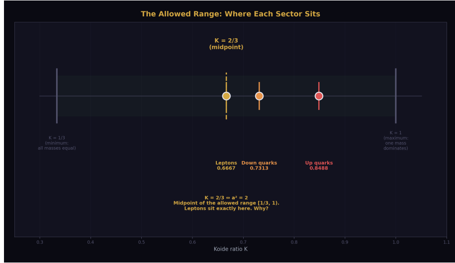
Figure 6: Fig. 7: Cauchy-Schwarz bounds 1/3 \leq K < 1 . K = 2/3 is the midpoint. Leptons sit exactly at the midpoint, down quarks at 0.73, up quarks at 0.85. Why do leptons sit at the midpoint?
