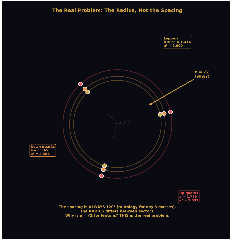
Figure 7: Fig. 2: Three sectors on circles of different radii ( a = \sqrt{2}, 1.55, 1.76 ). The 120° spacing is always the same (tautology). The radius — why a = \sqrt{2} for leptons — is the unsolved problem.
