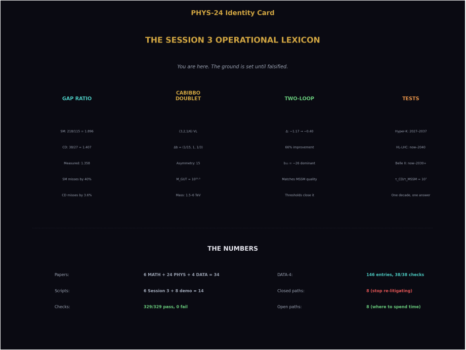
Figure 1: Fig. 8: The Session 3 operational ground — gap ratio (218/115 vs 38/27 vs 1.358), Cabibbo Doublet ((3,2,1/6), asymmetry 15), two-loop ( \Delta: -1.17 \rightarrow -0.40 ), 329/329 checks, the ground is set until falsified.
