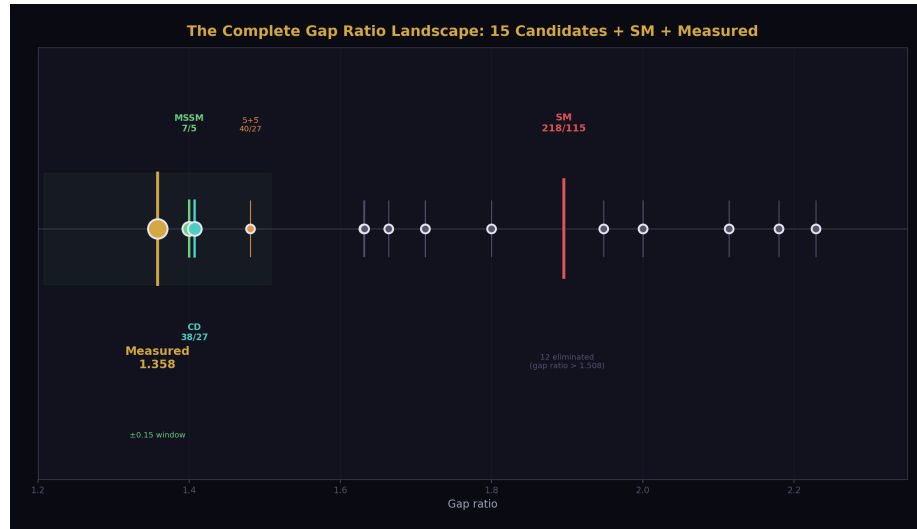
Figure 2: Fig. 4: All 15 candidates on one number line with the SM (218/115) and measured (1.358). Only MSSM (7/5) and the Cabibbo Doublet (38/27) survive within the \pm 0.15 window. 12 eliminated by arithmetic.
