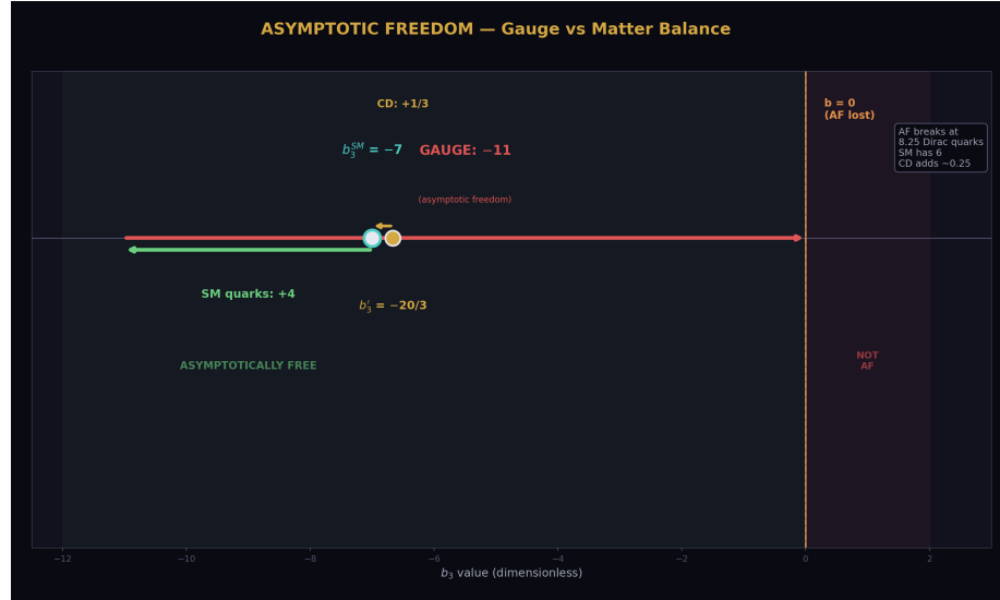
Figure 2: Fig. 5: The asymptotic freedom balance on a number line — gauge (-11) partially cancelled by matter (+4 \text{ SM}, +1/3 \text{ CD}) , leaving b_3' = -20/3 safely in the AF region.
