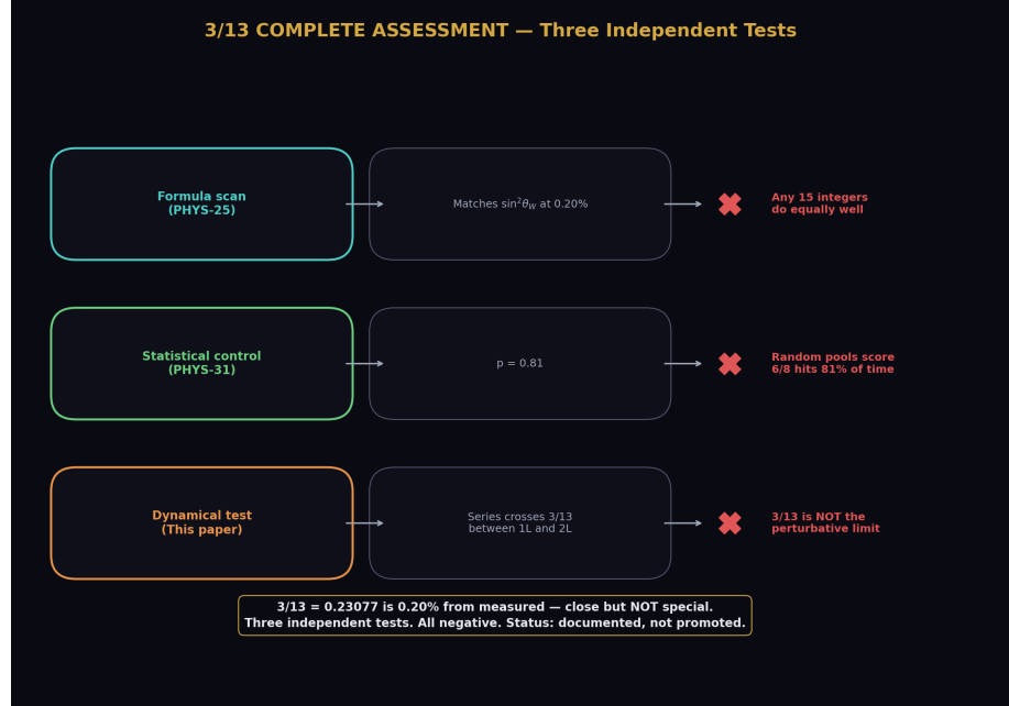
Figure 8: Fig. 8: Three independent tests of 3/13 — formula scan (not special), statistical control ( p=0.81 ), and dynamical test (series overshoots). All negative. 3/13 is documented but not promoted.
