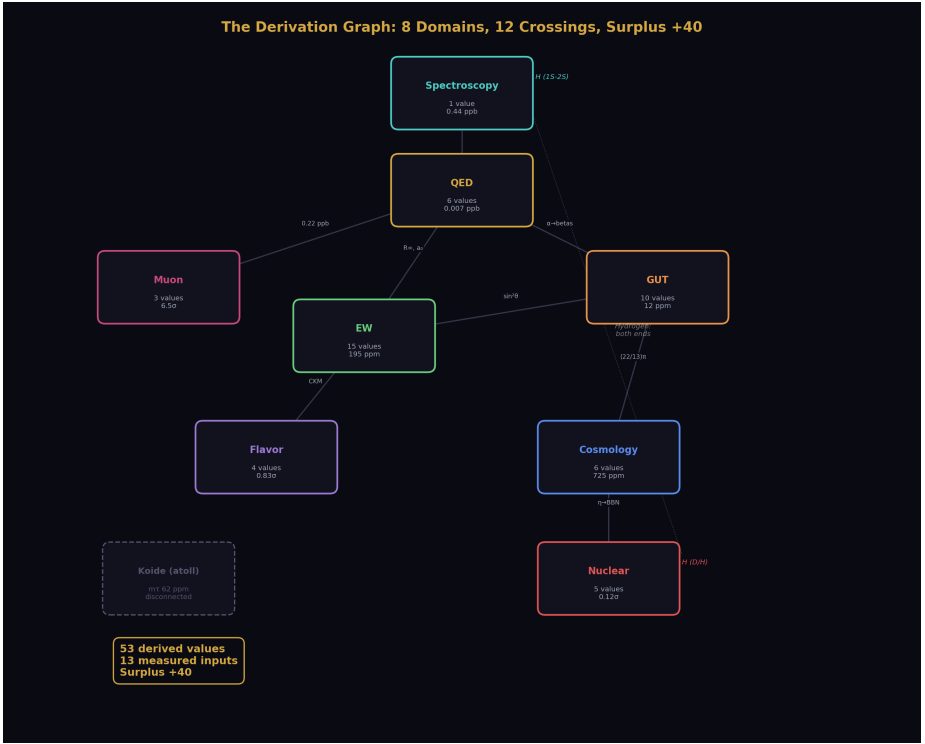
Figure 3: Fig. 5: Eight physics domains connected by twelve crossings — hydrogen appears at both ends, Koide atoll floats.
