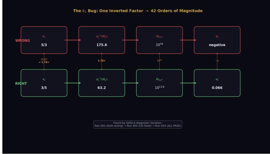
Figure 7: Fig. 7: The k_1 normalization bug — one inverted factor ( 5/3 vs 3/5 ) cascaded to 10^{42} error in M_{GUT} .
