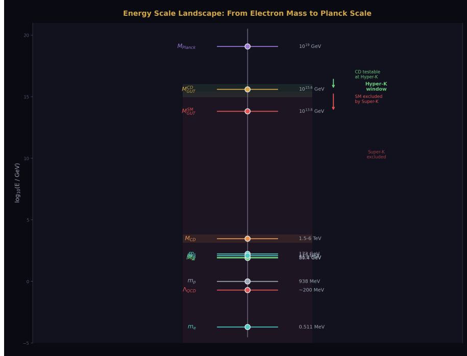
Figure 2: Fig. 3: Energy hierarchy from m_e to M_{\text{Planck}} — SM M_{\text{GUT}} excluded by Super-K, CD M_{\text{GUT}} in Hyper-K window.
