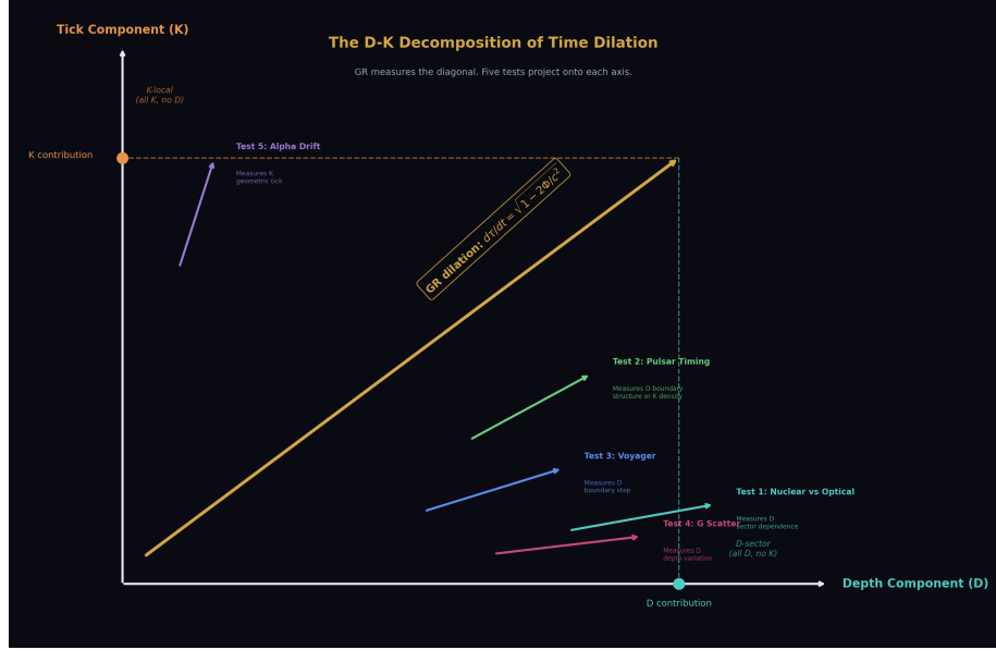
Figure 2: Fig. 1: The D-K Decomposition — GR measures the diagonal. Five tests project onto Depth and Tick axes.
