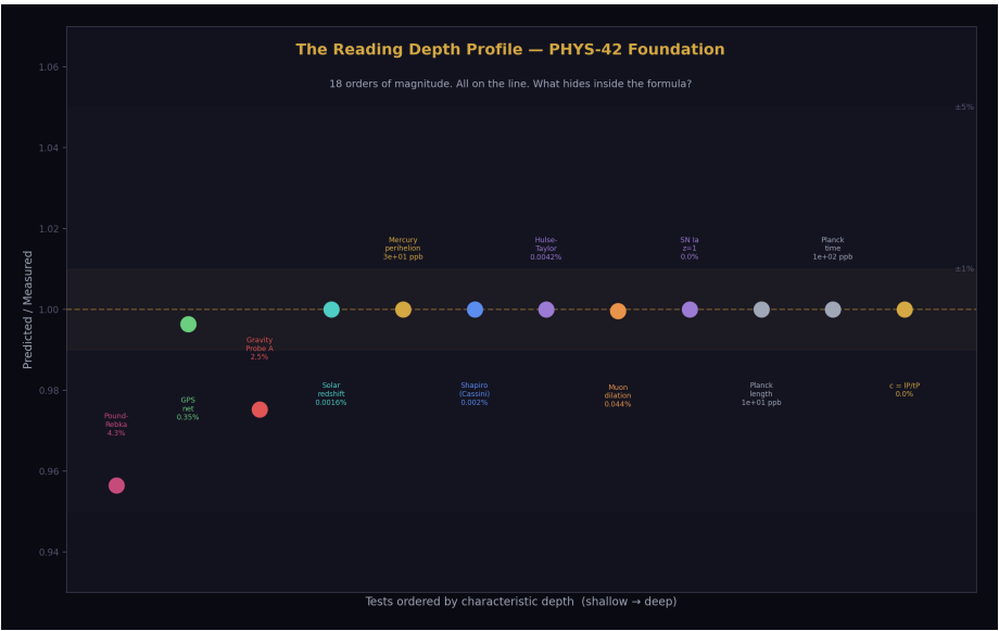
Figure 1: Fig. 2: PHYS-42 confirmation across 18 orders of magnitude. All on the line. What hides inside?
