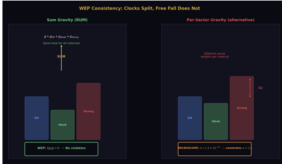
Figure 7: Fig. 8: Sum gravity (left) produces no WEP violation — all materials fall the same. Per-sector gravity (right) is constrained by MICROSCOPE. RUM predicts sum gravity: clocks split by sector, free fall does not.
