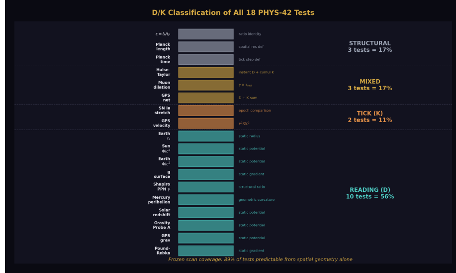
Figure 2: Fig. 2: All 18 tests classified as Reading (D), Tick (K), Mixed, or Structural. D dominates at 56%. Frozen scan covers 89%.
