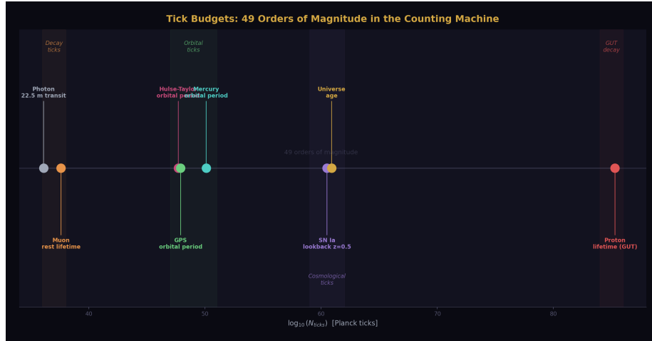
Figure 3: Fig. 5: From photon transit ( 10^{36} ticks) to proton lifetime ( 10^{85} ticks). Three regimes: decay, orbital, cosmological. The counting machine spans 49 orders.
