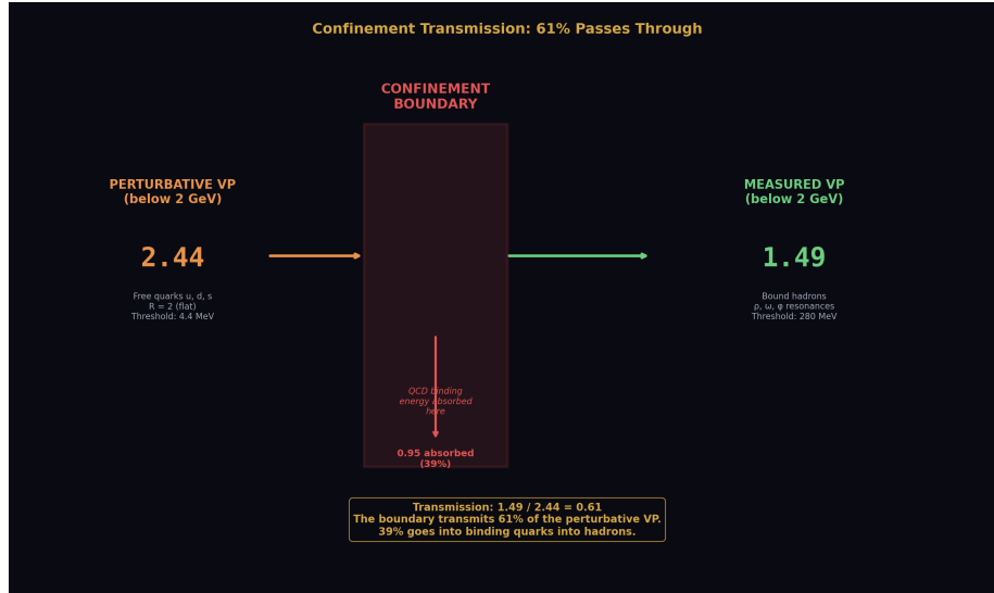
Figure 3: Fig. 4: Perturbative VP (2.44) enters the confinement boundary — 1.49 (61%) emerges as measured VP, 0.95 (39%) absorbed by binding energy.
