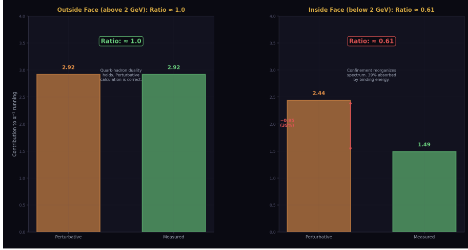
Figure 1: Fig. 5: Above 2 GeV (outside face): perturbative matches measured, ratio \approx 1.0 . Below 2 GeV (inside face): perturbative exceeds measured, ratio \approx 0.61 .
