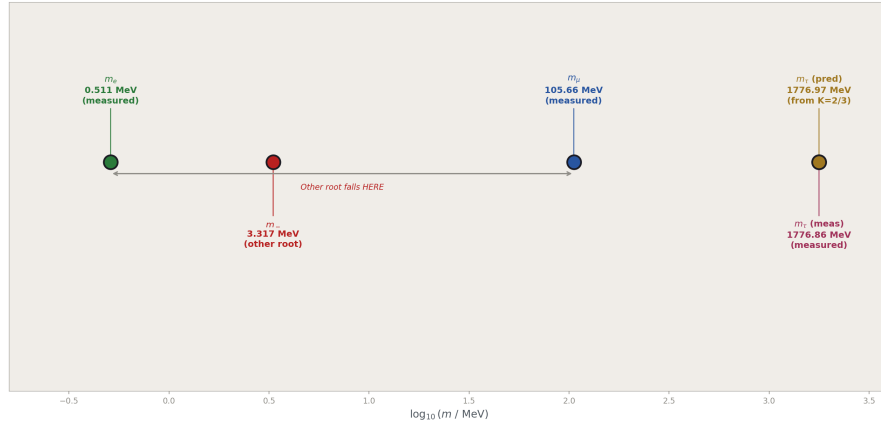
Figure 6: Fig. 4: The charged lepton masses on a log scale with the Koide prediction (gold) at the measured tau position and the other quadratic root (red) between electron and muon.
